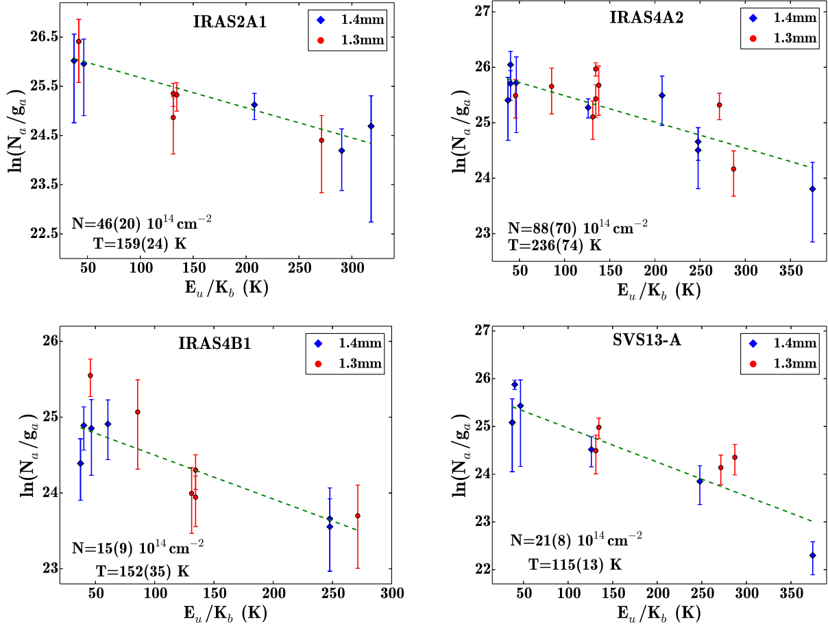
Fig. 3. Rotation diagram for the glycolaldehyde transitions reported in Table 2 for NGC 1333-IRAS2A (upper-left panel), NGC 1333-IRAS4A2 (upper-right panel), NGC 1333-IRAS4B1 (lower-left panel), and NGC 1333-SVS13A (lower-right panel). The line intensities have been corrected for beam dilution using the sizes derived in Sect. 4.1. The parameters N_{\text{up}} , g_{\text{up}} , and E_{\text{up}} are respectively the column density, the degeneracy, and the energy of the upper level. The error bars on \ln(N_{\text{up}}/g_{\text{up}}) are given by the vertical bar of the symbols. Red and blue points refer to the lines detected in the 1.3 mm and 1.4 mm spectral bands, respectively. The dashed lines represent the best fits.
