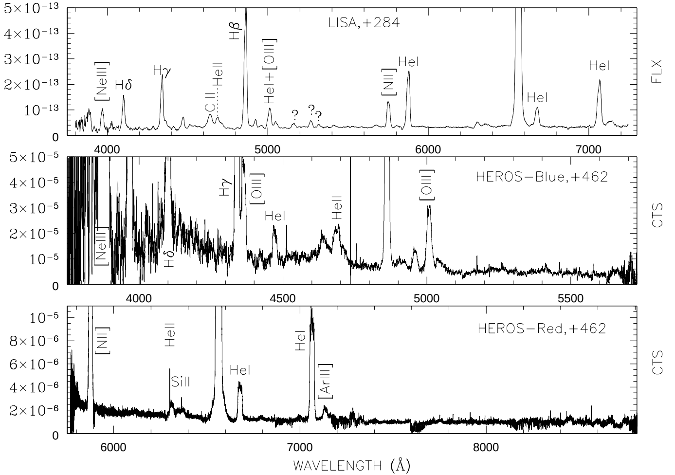
Fig. 11. LISA (top panel) and HEROS (mid and bottom panels) spectra of 17hx \sim 1 yr after outburst and/or discovery. The LISA spectrum is in units of \text{erg cm}^{-2} \text{s}^{-1} \text{\AA}^{-1} and uncorrected for reddening, while the HEROS spectrum is in arbitrary units. The spectrograph and the age of the spectrum are indicated in each panel.
