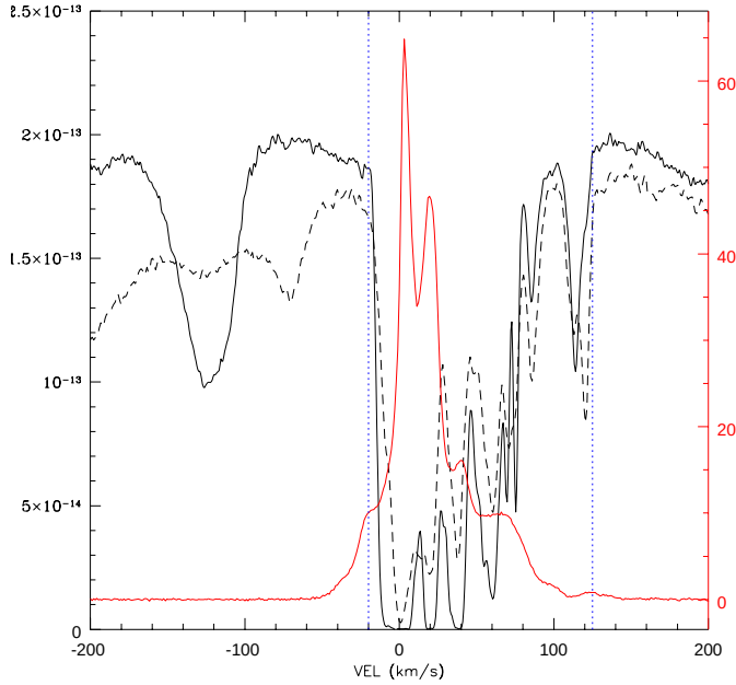
Fig. 2. Comparison of the temperature profile of the H I 21 cm (red line) with the Na I (black solid line) and Ca II K (black dashed line) interstellar absorption profiles. The two vertical blue dotted lines mark the limits for the column density calculation (see Sect. 2 for details). Units of flux ( \text{erg s}^{-1} \text{cm}^{-2} \text{\AA}^{-1} ) and temperature (K) are on the left and right axis, respectively.
