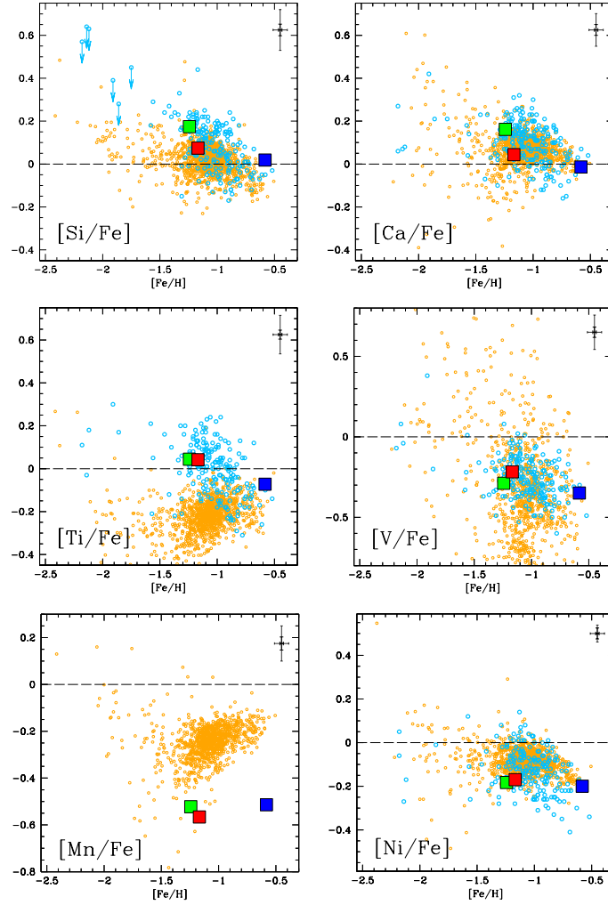
Fig. B.1. Behaviour of [Si/Fe], [Ca/Fe], [Ti/Fe], [V/Fe], [Mn/Fe] and [Ni/Fe] as a function of [Fe/H] for the three SMC target clusters (squares, same colours in Fig. 1), SMC field stars of Paper I (cyan circles) and SMC field stars measured by APOGEE (orange circles).
