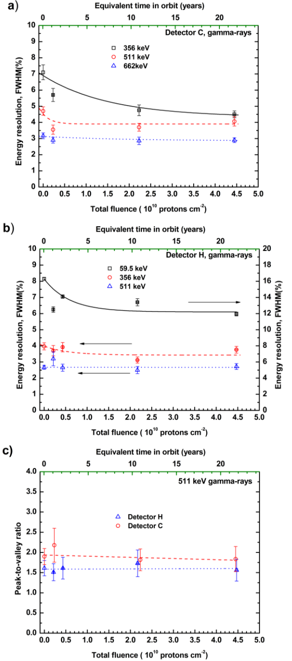
Fig. 7. Energy resolution versus the total proton fluence for several \gamma -ray lines with the CdTe detectors. (a) Detector C. (b) Detector H. Lines: the exponential decay fits applied to the data, just for guideline purposes. (c) Peak-to-valley ratio for the 511-keV line versus the total proton fluence, with detectors C and H. Lines: the linear fits applied to the data. V_{\text{bias}} = -140 \text{ V} and 1\text{-}\mu\text{s} shaping time.
