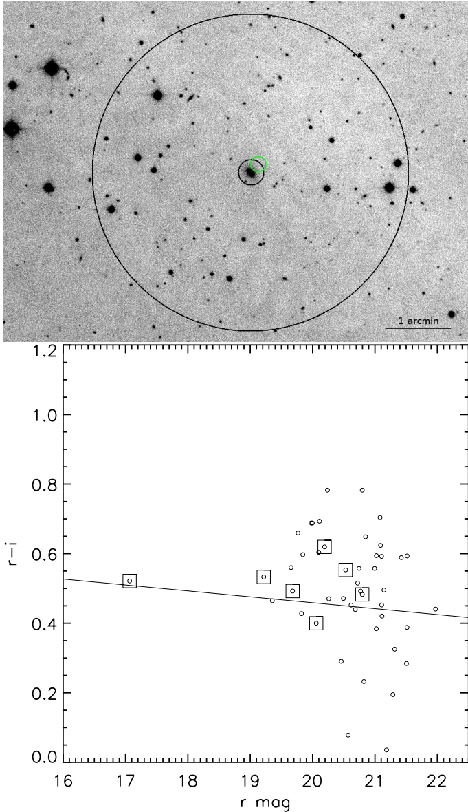
Fig. 8. PSZ1 G118.06+31.10, a galaxy cluster classified as fossil group following the definition of Voevodkin et al. (2010) . Top : WFC/INT r' band image of the cluster. The Planck pointing is shown with a small green circle, and the large circle has 5' diameter. The BCG is also highlighted. Bottom : colour–magnitude diagram of the galaxies near the cluster centre. The squares indicate the spectroscopically confirmed members within 0.5 Mpc distance from the BCG.
