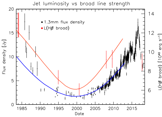
Figure 8. The blue curve is a fourth-order polynomial fit to the 1.3 mm light curve, F_{225}(t) . Notice that it underestimates the data before 1988 due to the flux from the secondary component during the strong flare. The orange curve is L(H\beta)(t) = \left[ \frac{F_{225}(t)}{1.8 \text{ Jy}} \right]^{0.4} 6.2 \times 10^{40} \text{ erg s}^{-1} . See the text for further discussion. Based on Equation (16), F_{225}(t) scales with the strength of the ionizing continuum.
