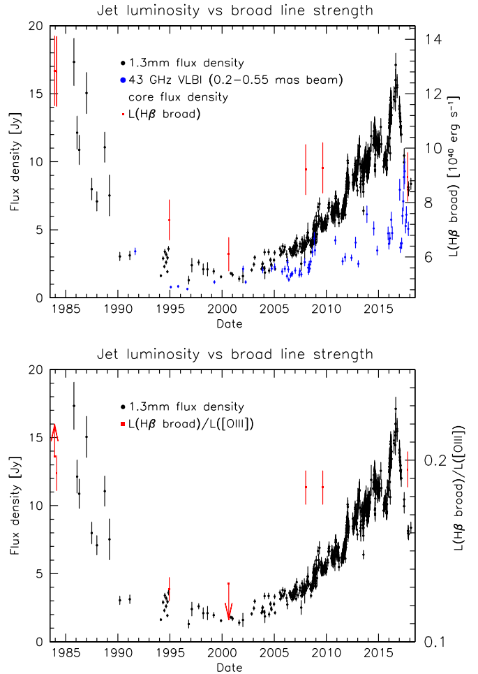
Figure 7. The top frame is a plot of the 225 and 43 GHz VLBI core flux densities vs. BEL luminosity from Table 1. The bottom frame shows the 225 GHz light curve and the L(\text{H}\beta) points from the top frame normalized by L([\text{O III}]\lambda 5007) in a 6 (\text{arcsec})^2 extraction region.
