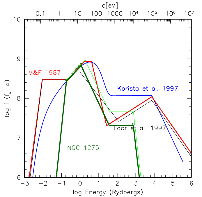
Figure 5. Comparison of the ionizing continuum inferred for NGC 1275 from the last subsection compared to other popular ionizing continua used in the literature as input spectra for CLOUDY simulations of AGN BELs (Mathews & Ferland 1987; Korista et al. 1997; Laor et al. 1997). The ionizing spectrum of NGC 1275 in green is softer.
