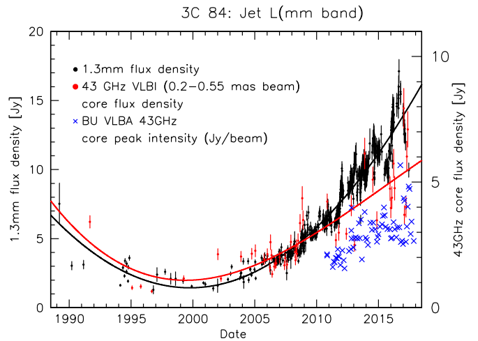
Figure 6. A comparison of the 1.3 mm flux density light curve and the 43 GHz VLBI core flux density light curve. The data covers a time span of \sim 1990 until spring 2017. The black curve and the red curves are the third-order polynomial fits to the 1.3 mm and 43 GHz VLBI data, respectively.
