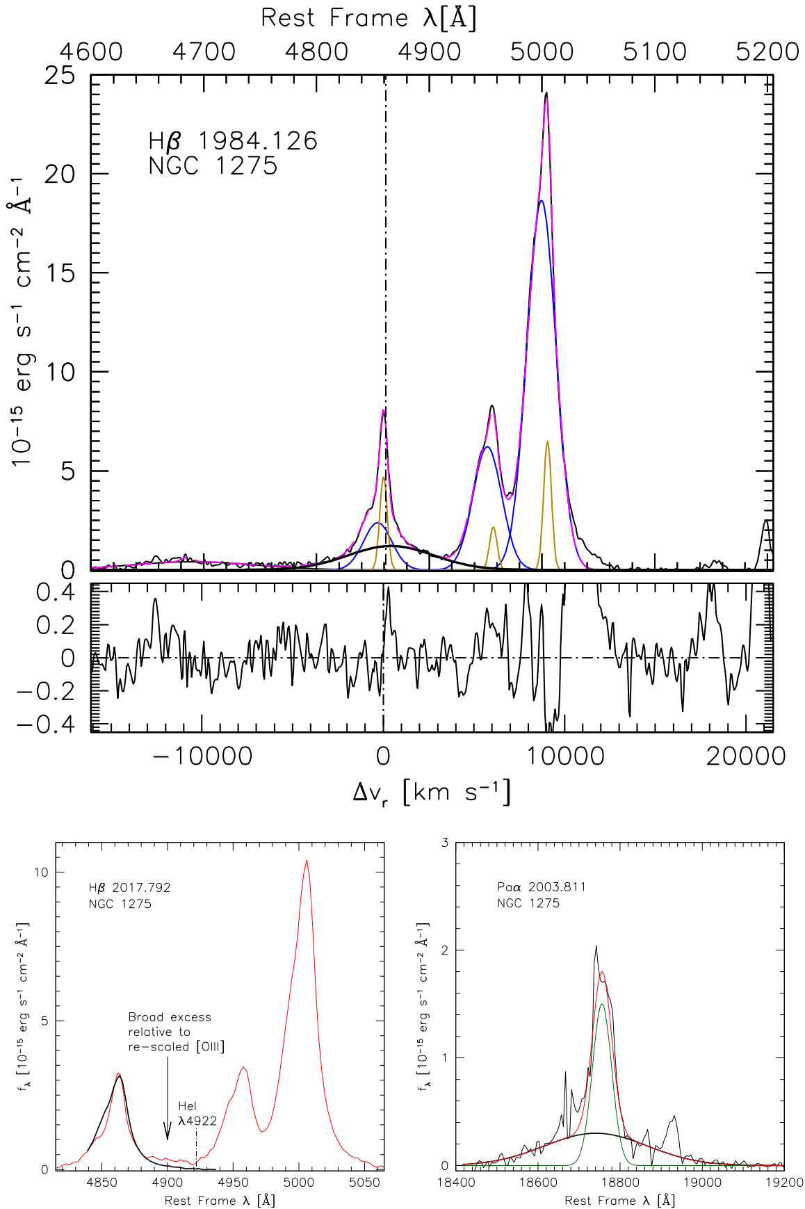
Figure 1. The top frame illustrates our fitting procedure for the H \beta and [O III] complex (epoch 1984.126) that is described in the text. The BEL, semi-broad NL, and NL (wind) are black, blue, and yellow, respectively. The bottom left frame shows the redwing excess of H \beta relative to a scaled [O III] NL profile. Note that there is no evidence of a weak He I \lambda 4922 emission line or the Fe II \lambda 4924 emission line. The bottom right frame shows the BEL (NL) in Pa \alpha in brown (green).
