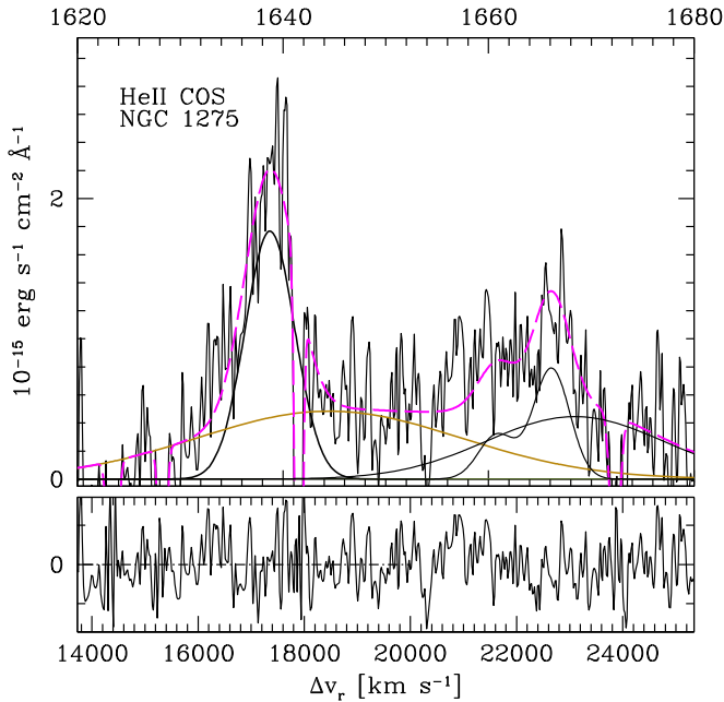
Figure 4. Low ionization parameter simulations predict a strong He II \lambda 1640 BEL relative to the nearby C IV BEL. The fit is fairly complicated. There are narrow and broad (brown) He II lines and a broad Al II \lambda 1671 line. In addition there are the two NLs O III \lambda 1666 and O III \lambda 1663 that are fit in a 2.5:1 ratio. The estimate of the He II BEL line strength is recorded in Table 1.
