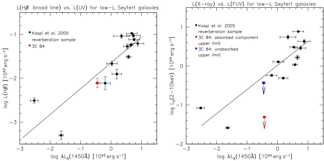
Figure 3. Diagnostics of the photoionizing continuum. The left frame shows that 3C 84 has a far-UV-H \beta ratio similar to that of weak broad line Seyfert galaxies. The right frame indicates that the ionizing continuum is softer than a typical broad line Seyfert galaxy of similar far-UV luminosity. The unabsorbed Chandra estimate is a very loose upper bound as discussed in the text. The lines are the best-fit power laws to the Kaspi et al. (2005) data.
