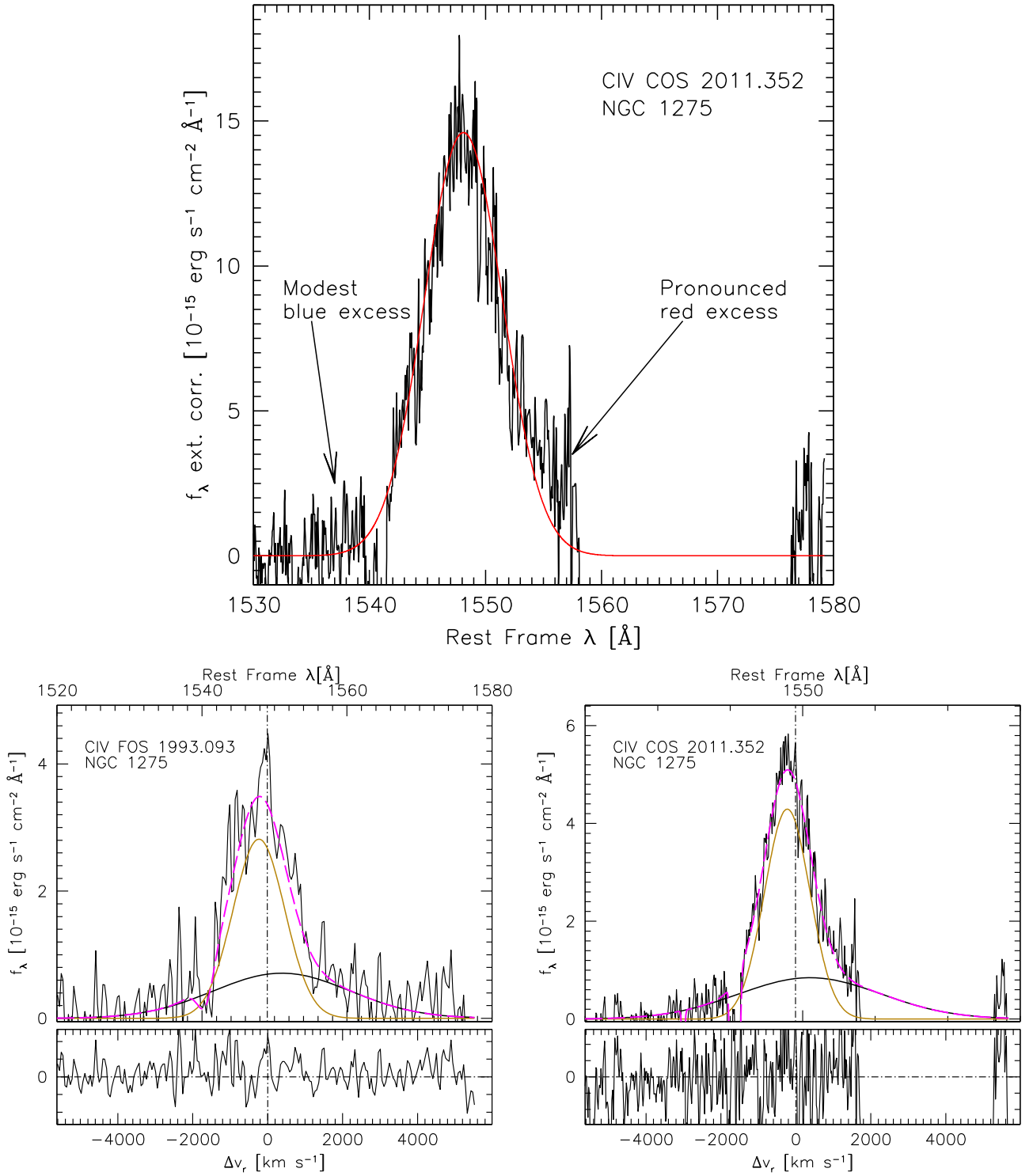
Figure 2. The top frame illustrates that the widest plausible NL fit to C IV in 2011.352 still results in a significant red wing residual. The bottom frame fits the C IV profile with a NL+BEL in 1993.093 (left) and 2011.352 (right).
