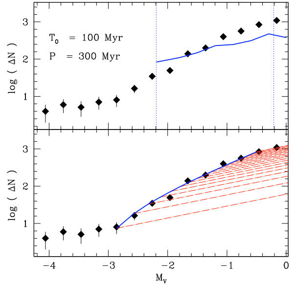
Fig. 2. Lower panel: logarithmic integrated LF of young MS stars (filled diamonds). The LF is reproduced by the sum (thick continuous line) of 20 LFs (dot-dashed lines) of simple stellar populations. It is assumed here that the slope of the single LFs is equal to that of NGC 2004 (a young populous cluster of the Large Magellanic Cloud; \alpha = 0.32 \pm 0.04 , see Fig. 13 in SHR04) and that the simple stellar population contains 0.5 times the number of stars in NGC 2004. The populations were generated at a constant rate during \sim 273 Myr (see Sect. 3.1), and all stars now evolved off the main sequence were removed from the LFs. Upper panel: the observed LF (filled diamonds) compared with a synthetic one (thick continuous line) generated with a bursting star formation. The epoch of the last episode ( T_0 ) and the time lapse between the star formation episodes ( P ) are indicated. Dotted vertical lines mark the termination of the MS for the single bursts. See SHR04 and text for details.
