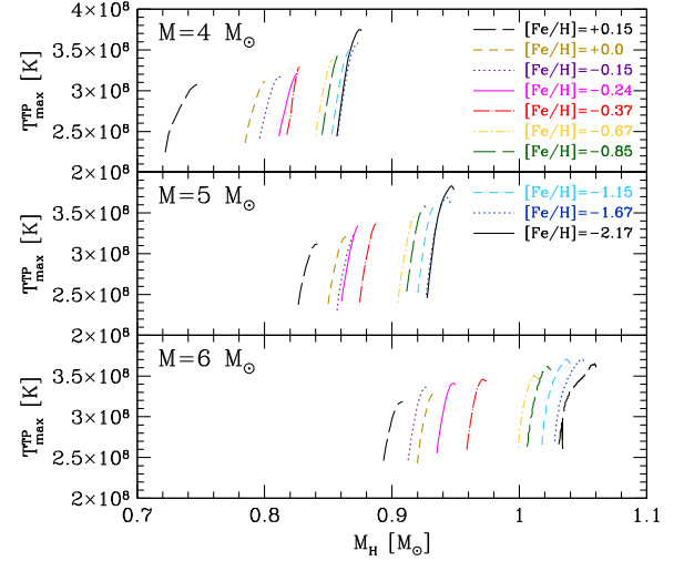
Figure 11. As in Figure 5, but for the maximum temperature attained at the bottom of the convective zone generated by a TP.
