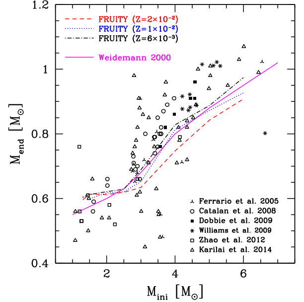
Figure 21. FRUITY models Initial-to-final mass relations for selected metallicities, compared to the semi-empirical relation from Weidmann (2000) and to Open Clusters observations.
