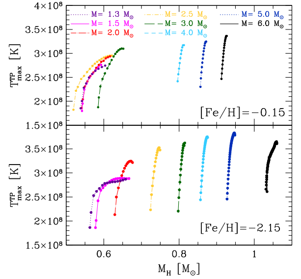
Figure 10. As in Figure 3, but for the maximum temperature attained at the bottom of the convective zone generated by a TP.
