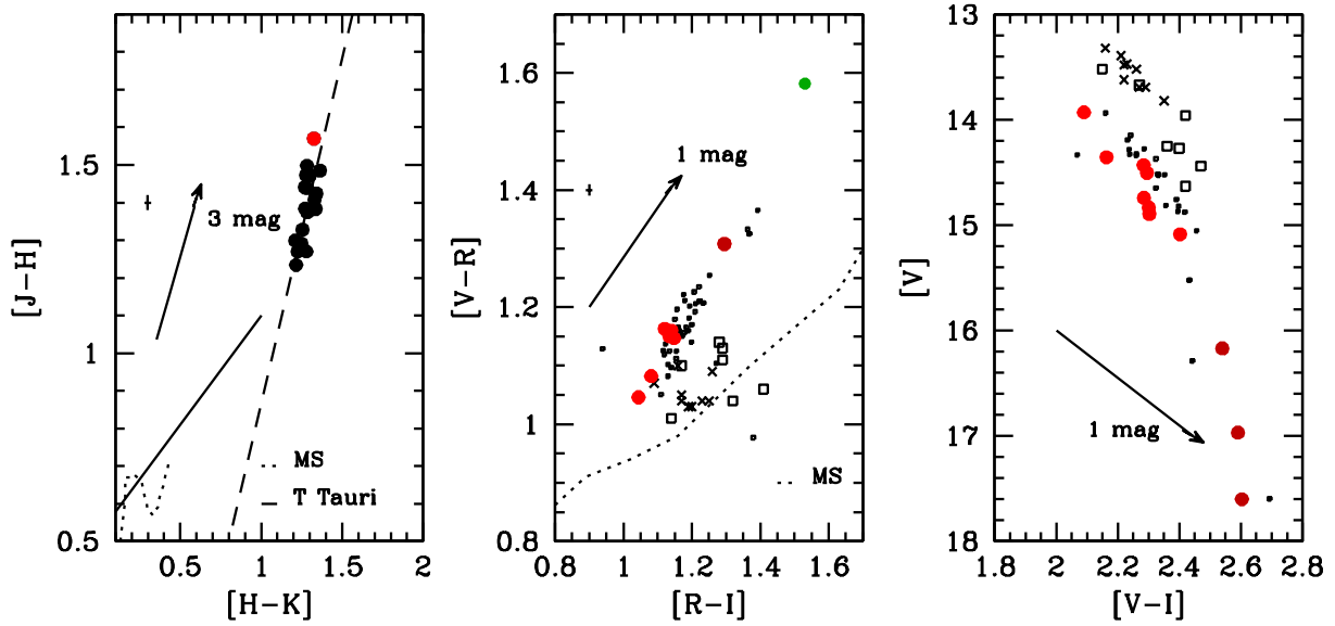
Fig. 6. Left panel: NIR two-color plot [J-H] vs. [H-K] . The red point represents the NIR colors at MJD = 57 662 (see text). Continuous line: locus of T Tauri stars (Meyer et al. 1997). Dotted line: unreddened main-sequence. Dashed line: linear fit through the data. Arrow: extinction vector corresponding to A_V = 3 mag (reddening law of Cardelli et al. 1989). The average error is indicated with a cross. Middle panel: optical two-color plot [V-R] vs. [R-I] . Arrow: extinction vector corresponding to A_V = 1 mag. Dotted line: unreddened main-sequence. Red and dark-red large dots: our data taken before and after June 2017. The green dot represents the colors of 2015 June 22 (AAVSO database). Black data: literature/AAVSO data with the same symbols as in Fig. 1. Right panel: [V] vs. [V-I] . Symbols and colors as in the middle panel.
