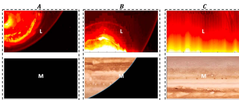
Figure 1. Examples of L band data and contamination (top) function of M channel pointing (bottom, graphic art). (a) South Aurora, very low contamination, M band FoV is pointing toward empty space. (b) South Aurora, medium contamination in the bottom of the image; M band FoV is partially filled by Jupiter. (c) North Aurora, very high contamination, M band FoV is completely filled by Jupiter.
