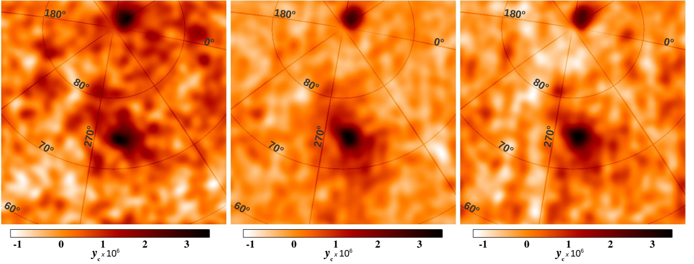
Fig. 4. Left to right: individual SZ maps at 70, 100, and 143 GHz in units of 10^6 times the Compton parameter. The field of view is 31^\circ 9' and the coordinates are Galactic. Virgo is the extended source below the centre. The Coma cluster is also clearly visible in the top of the map. The maps have been smoothed to a resolution of 1.5' to highlight the faintest structures.
