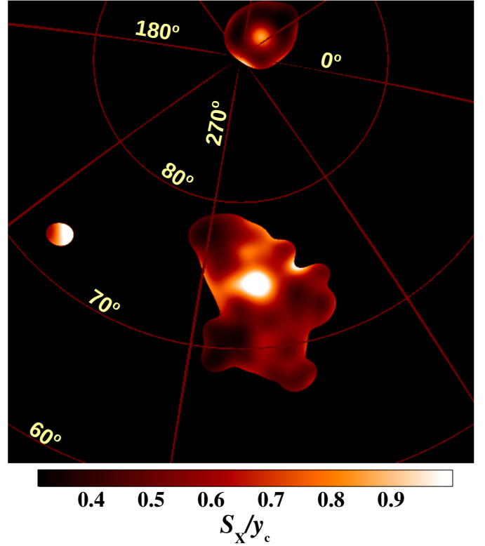
Fig. 11. Ratio between ROSAT and Planck data (smoothed to 1.5' ). The ratio S_X/y_c is defined only in regions with sufficient SZ signal (the smoothed signal is larger than 1.5 times the dispersion of the map). Three clusters can be distinguished in this plot, Coma in the north, Virgo in the centre, and Leo in the east. The ratio is normalized to 1 at the maximum.
