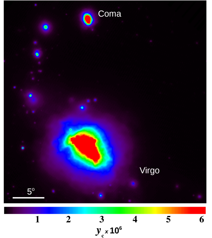
Fig. 1. Simulated Virgo cluster from a constrained simulation in units of 10^{-6} times the Compton parameter (Dolag et al., 2005). To increase the contrast, the Compton parameter beyond 6 \times 10^{-6} has been saturated. The brightest cluster in the top is Coma. In this and other figures (unless otherwise noted) the coordinates are Galactic, the projection is orthographic, and the field of view is 31.94 across or 8.3 (11.9) Mpc assuming Virgo is at a distance of 15 (21.4) Mpc. The North Galactic pole is up and Virgo's centre (M87) is 4^\circ south of the centre of the images.
