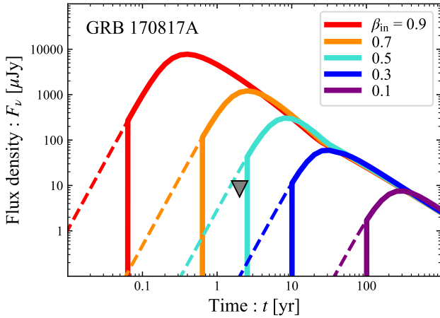
Figure 7. The same as Figure 3 but for GRB 170817A. The adopted parameters are E_{ej} = 10^{51} erg, n = 2 \times 10^{-3} \text{ cm}^{-3} , \epsilon_B = 0.1 , p = 2.5 , \bar{\epsilon}_e = 0.1 , and E_j = 10^{49} erg.
