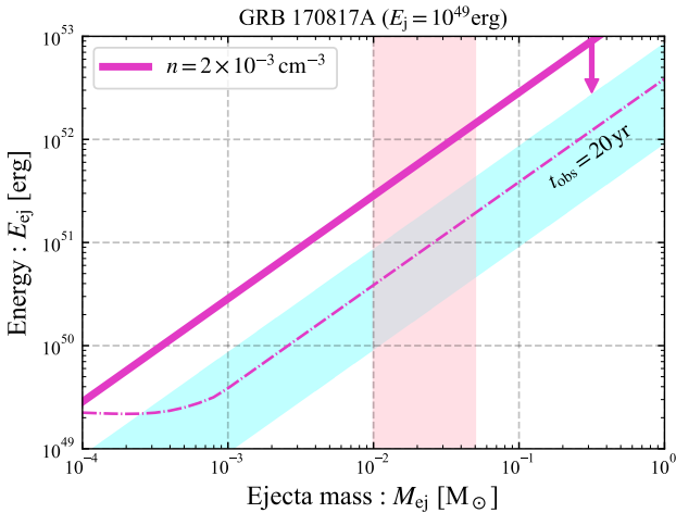
Figure 8. The same as Figure 6 but for GRB 170817A. The pink and cyan shaded regions show the range of ejecta mass M_{ej} = 0.01 - 0.05 M_\odot and velocity \beta_{in} = 0.1 - 0.3 , respectively. The dash-dotted curve demonstrates how we can reduce the allowed region by late-time observations (e.g. Butler et al. 2018).
