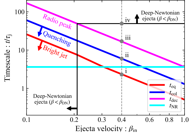
Figure 2. Normalized timescales as a function of \beta_{in} , the ejecta initial velocity for E_{ej}/E_j = 100 . The horizontal cyan line depicts t_{NR} , the transition time of the jet to Newtonian regime. The radio flare peaks on the magenta line and it declines (rises) above (below) this line. Below the blue line, the emission from the ejecta is quenched by the jet. On the red line, the (unperturbed) ejecta signature would have been equal to the jet afterglow and the latter dominates below this line. The dashed vertical line outlines the behaviour of the light curve for a given initial velocity ( \beta_{in} = 0.4 ). At early time below (i) the afterglow radio signal dominates. Between (i) and (ii) the jet blast-wave that has expanded to a quasi-spherical structure quenches the ejecta radio signal. The ejecta collides with the jet blast-wave at (ii) and from that time on its interaction with the ISM produces a radio light curve peaks at (iii). It undergoes a transition to the deep-Newtonian regime at (iv).
