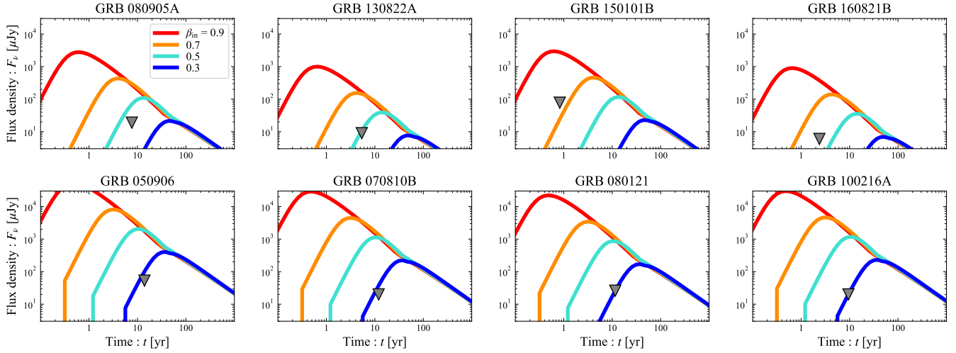
Figure 5. Radio light curves for E_{ej} = 10^{52} erg, n = 10^{-2} \text{ cm}^{-3} , \varepsilon_B = 0.1 , and different velocities, corresponding to ejecta masses of M_{ej} \approx 0.004 M_\odot (red), 0.014 M_\odot (orange), 0.036 M_\odot (cyan) and 0.12 M_\odot (blue). The other parameters are p = 2.5 and \bar{\varepsilon}_e = 0.1 . The top panels show cosmological events with z \leq 0.1 and the bottom panels show candidate local ( < 200 Mpc) events. The gray triangle shows the measured upper limit, where we report only the most constraining value if several observations are available.
