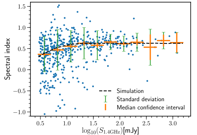
Fig. 3. Spectral index distribution of the radio-AGN galaxies with both LoTSS and 1.4 GHz measurements, as a function of 1.4 GHz flux density. Individual sources are shown as blue dots and the medians of different bins in 1.4 GHz flux density are shown as orange crosses. The vertical lines correspond to the standard deviation on each bin. The median spectral index at flux densities S_{1.4\text{GHz}} > 20\text{ mJy} is 0.63. The weak decrease in median spectral index at lower flux densities may be driven by selection biases in the 1.4 GHz sample, as indicated by the black dashed line that simulates the effect of this (see text for details).
