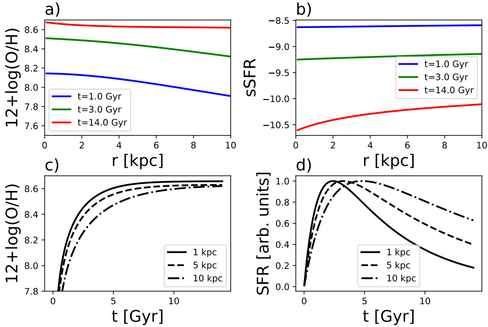
Figure 4. a) The time evolution of the metallicity radial profile using the v \propto V/r model and parameter values (a, b, \nu_0, \lambda) = (5.0, 2.0, 0.5, 1.0) . b) Time evolution of the sSFR radial profile for the same model. c) Time evolution of the ISM metallicity at three different galactocentric distances, as noted in the legend. d) The star formation histories of three regions at different galactocentric distances. Each SFH is normalised to its maximum value. The panel demonstrates out prescription for inside-out growth, where outer regions form stars later and more slowly.
