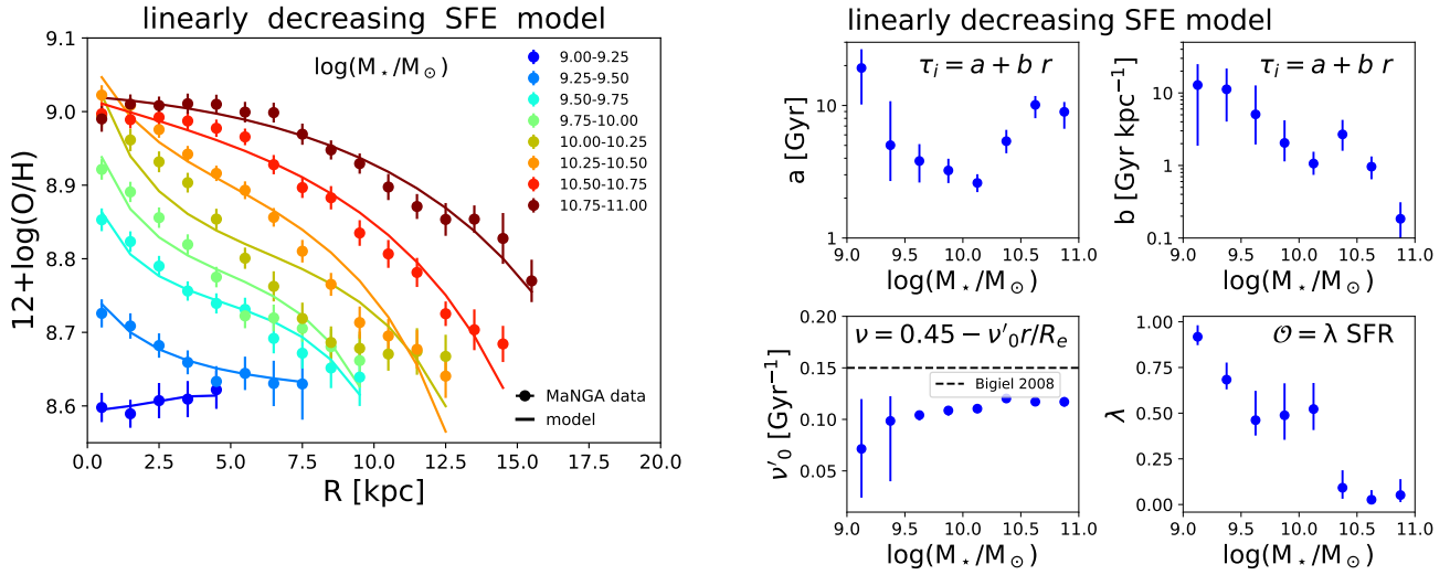
Figure 9. Left: Same as Fig. 7, but using the linearly decreasing SFE model. Right: Same as Fig. 8, but using the linearly decreasing SFE model. The parameter \nu'_0 denotes the linear slope of the SFE and is compared to the median value obtained analyzing the data from Bigiel et al. (2008) for a small sample of local star forming galaxies.
