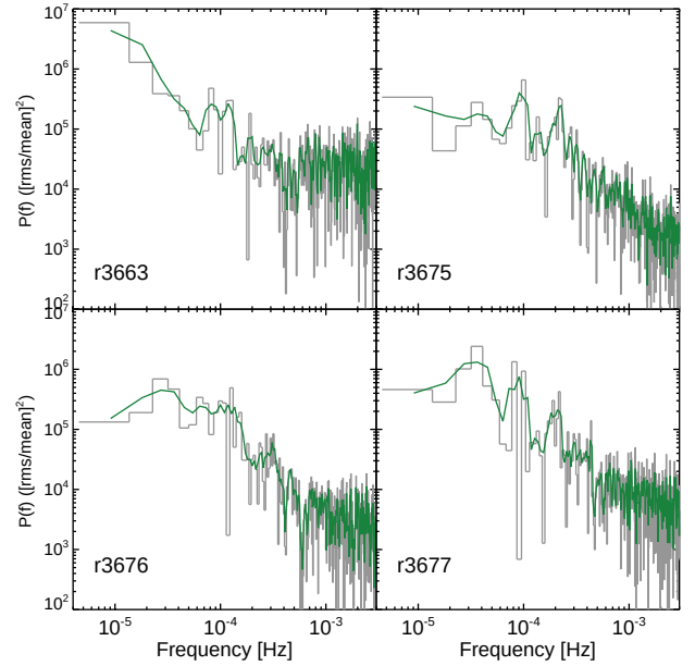
Figure 4. Periodograms for the hard band dipping observations (without Poisson noise subtraction). The green curve is the Gaussian smoothed periodogram over n = 3 neighbouring bins.
