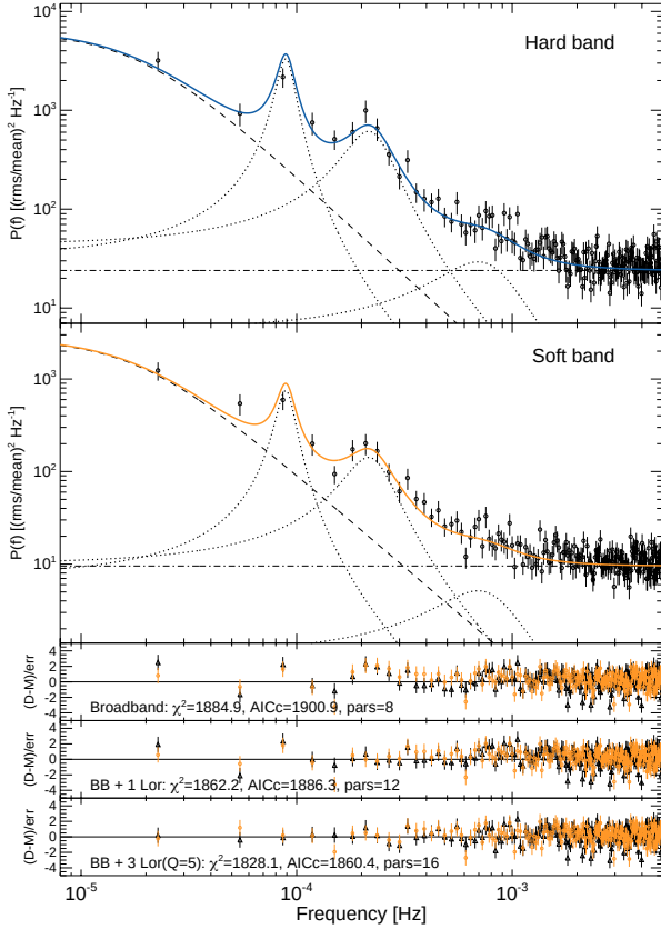
Figure 3. PSD modelling of the dipping observations using multiple Lorentzian components. The best fit model (BB+3Lor( Q_{l_1} = 5 )) with a zero-centered Lorentzian (dashed) and three additional narrower Lorentzians (dotted) are shown for the hard and soft bands in the upper and middle panels respectively. The horizontal dot-dashed line is the Poisson noise parameter. The lower three panels show the standard residuals for this and two less complex models.
