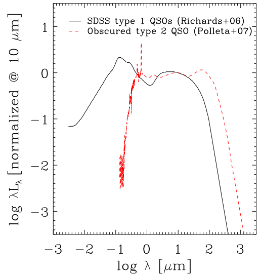
Figure 1. The SED templates adopted in this work to describe the emission of SMBH particles. In our standard computations, we used the mean SED of SDSS type 1 quasars by Richards et al. (2006, black solid line). To check the stability of our results on the IR properties of clusters, we used the very different typical SED of an obscured type 2 QSO, reported by Polletta et al. (2007, red-dashed line).
