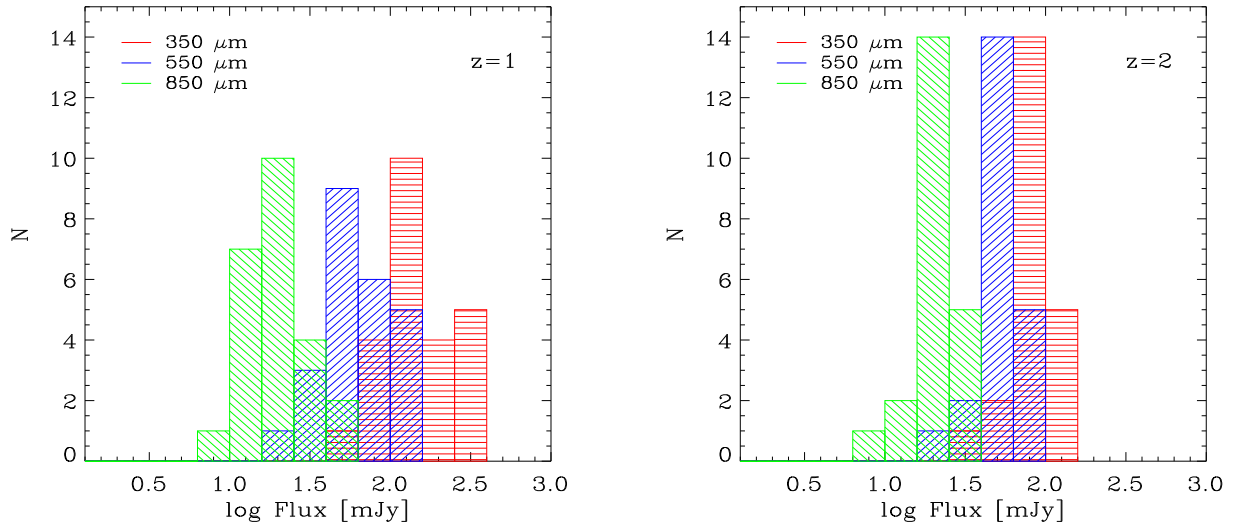
Figure 7. Distributions of the predicted fluxes from our sample of simulated clusters, within the Planck beam ( \sim 5 arcmin FWHM) in the 350, 550 and 850 \mu\text{m} HFI bands (857, 545 and 353 GHz, respectively). The four candidate protoclusters selected by Clements et al. (2014) have photometric redshift of 0.76, 1.04, 2.05 and 2.26 and 350 \mu\text{m} HFI fluxes of 1100, 810, 1250 and 1240 mJy, i.e. close to the right bound of these plots. However, these fluxes are believed to be overestimated by a factor of 2 to 3 due to selection bias. See text for details and discussion.
