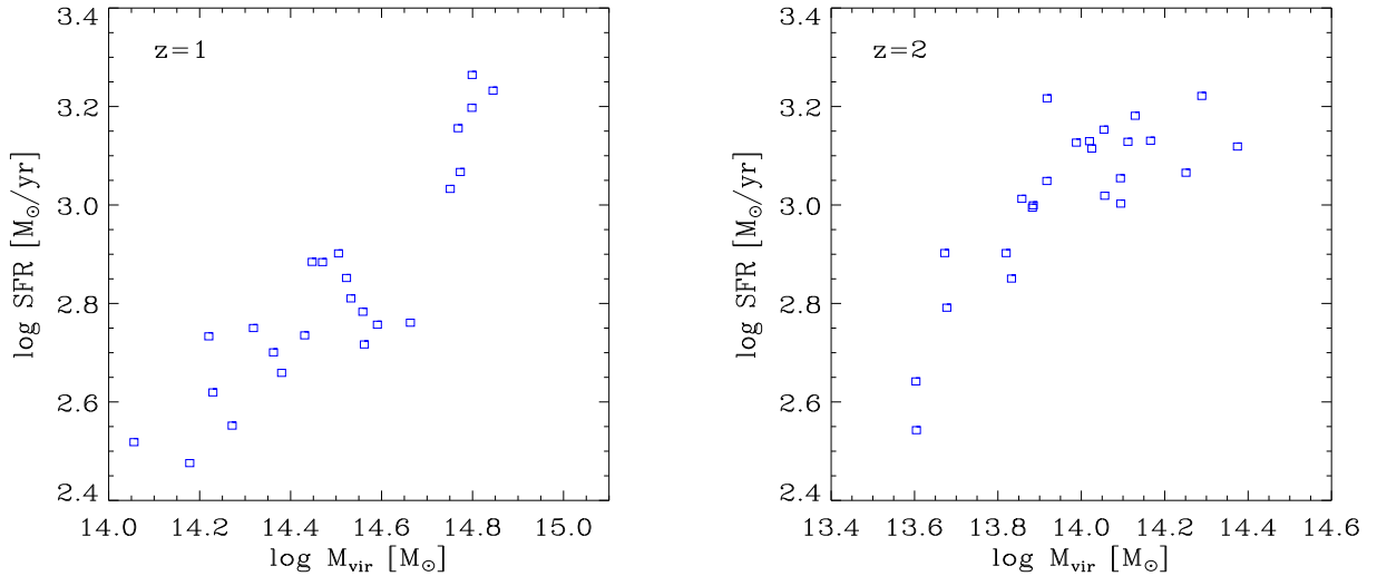
Figure 9. SFR as a function of virial mass for the sample of simulated clusters, at z = 1 (left) and z = 2 (right). The SFR is calculated including all gas particles within a box of 2000 kpc, close to the Planck HFI beam at both redshift.
