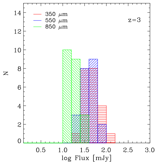
Figure 8. Same as Fig. 7, but at z = 3 .
