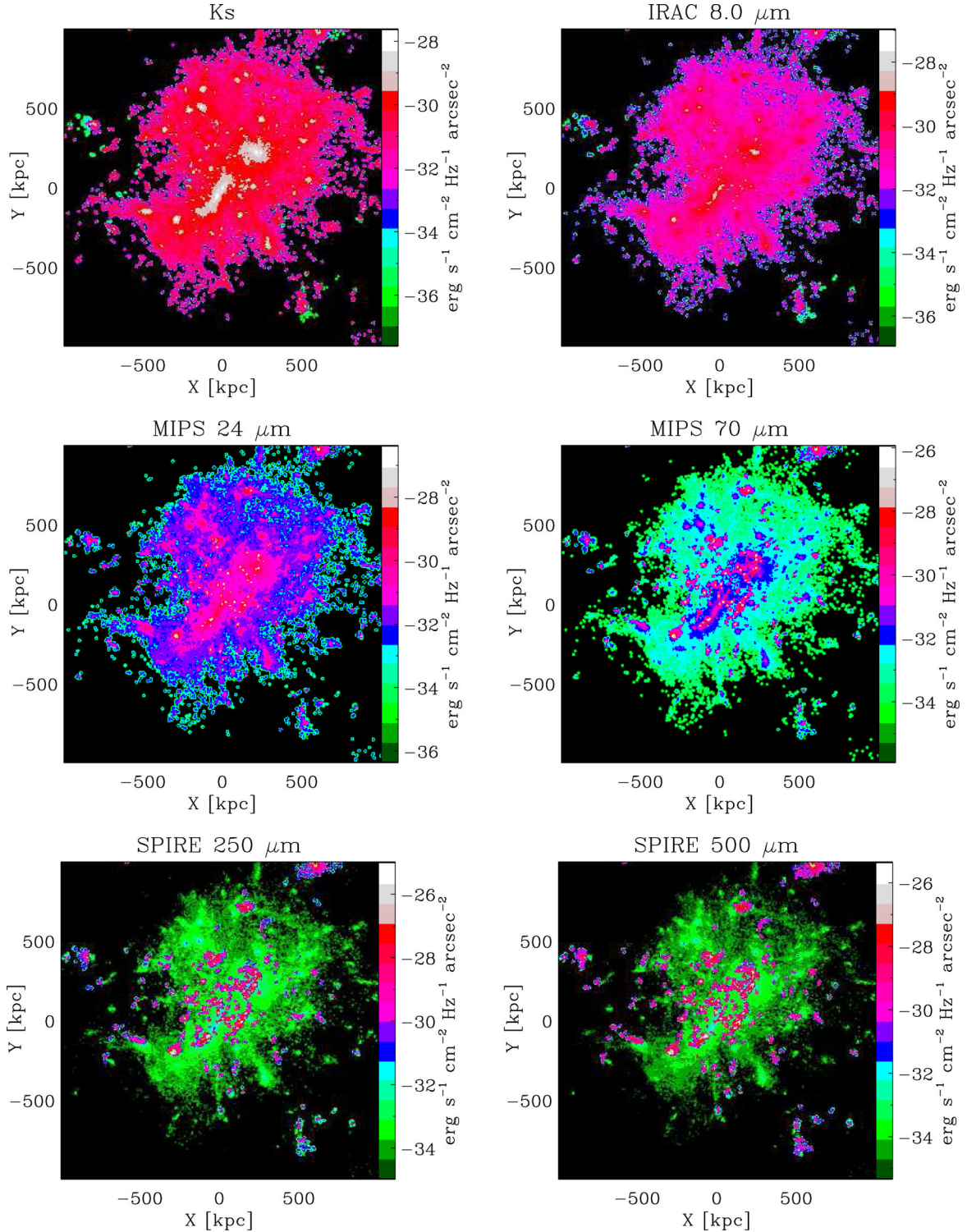
Figure 2. Examples of images of a cluster region at z = 1 produced by GRASIL-3D in various NIR to sub-mm bands. The physical size of each panel is 2000 kpc, close to the Planck HFI beam at that redshift. No telescope effects (like PSFs, pixel sizes, etc.) have been taken into account.
