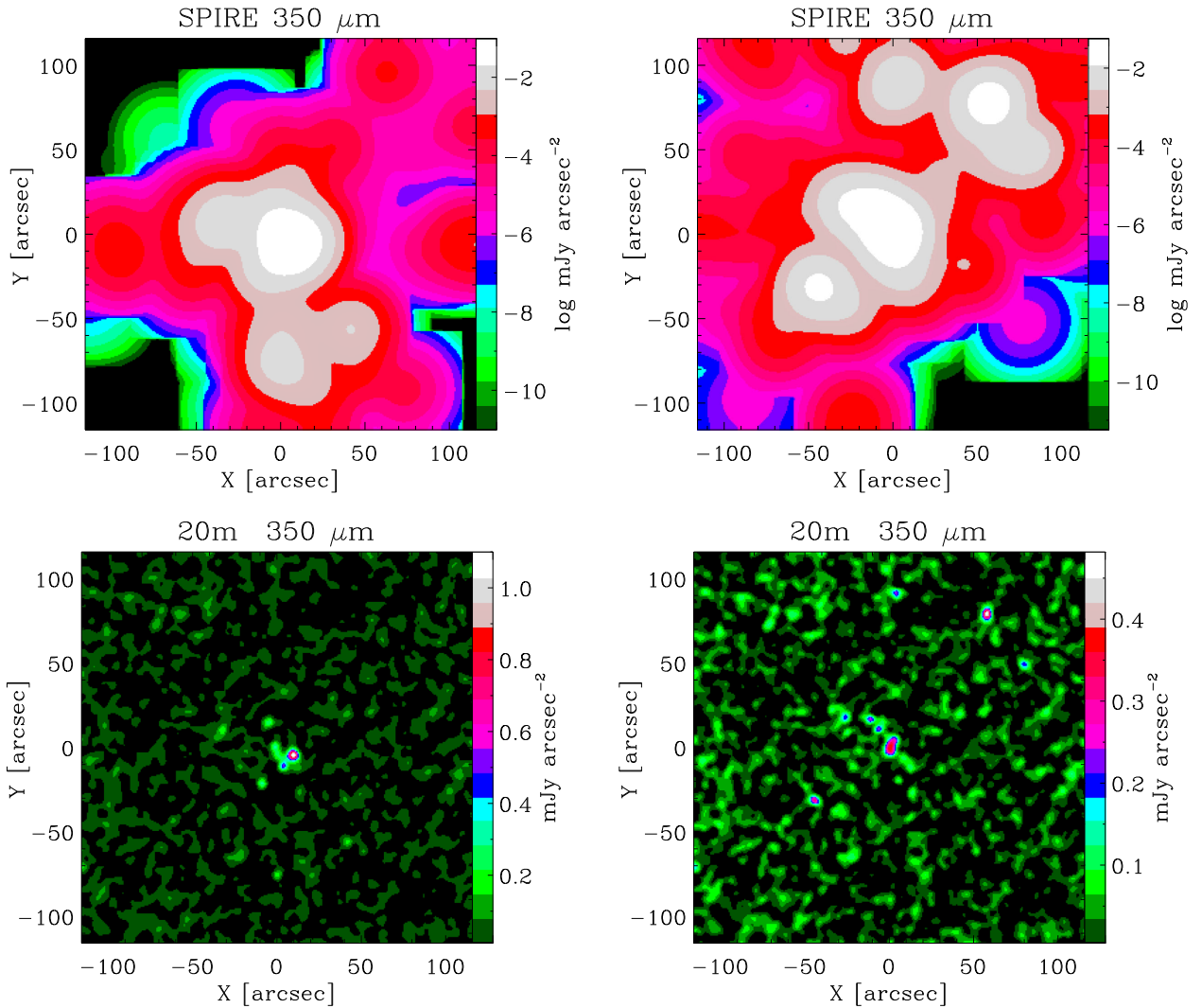
Figure 11. 350 \mu\text{m} (observed) GRASIL-3D images for the two cluster regions (left-hand and right-hand columns) at z = 2 having the highest SFR (at that redshift) in our sample, namely \sim 1600 \text{ M}_{\odot} \text{ yr}^{-1} within the box. The box physical size is 2000 kpc, close to the Planck HFI beam at z = 2 . The images in the top row have been convolved with a Gaussian PSF of 25 arcsec FWHM, corresponding to the Herschel telescope diffraction limit. We expect at most 2–3 individual sources with a flux in the beam above the Herschel confusion limit at this wavelength ( \sim 6 \text{ mJy} ). In the bottom row, the images include a Gaussian noise of 0.1 \text{ mJy arcsec}^{-2} 1\sigma , and are convolved with a PSF of 3.1 arcsec FWHM. This resolution can be achieved by a 20 m single dish telescope (see Sauvage et al. 2014).
