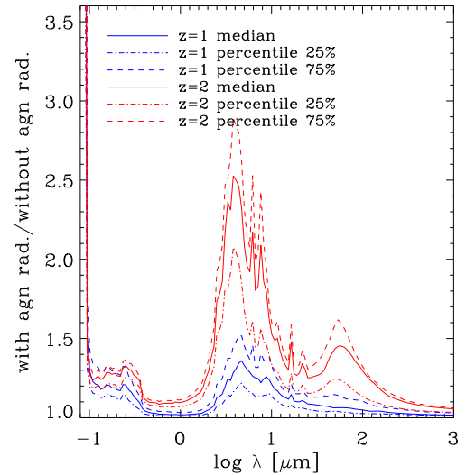
Figure 6. Ratio of the predicted fluxes including or excluding the radiative effect of AGNs, as a function of wavelength \lambda (rest frame), for our standard choice of GRASIL-3D parameters. Above \sim 100\text{ }\mu\text{m} the difference is in most cases \lesssim 25 per cent, decreasing with increasing \lambda .
