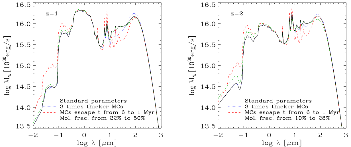
Figure 4. Comparison of the rest-frame SED obtained for one cluster at z = 1 and 2 , with different choices of GRASIL-3D parameters. Solid black: standard values; blue-dotted: increasing the mass of individual MCs (and thus their optical depth) by a factor of 3; red dashed: decreasing the escape time-scale of stars from MC by a factor of 6 (from 6 to 1 Myr); green dot-dashed: decreasing the threshold for gas to be in the dense MC phase by a factor of 10, so that the molecular gas fraction increases from about 22 per cent to about 50 per cent at z = 1 and from about 10 per cent to 28 per cent at z = 2 . In any case, the SEDs are very little affected above \lambda \gtrsim 100 \mu\text{m} , which is the spectral region on which we compare with observations in this paper. Note also that the parameter variations have been adopted to exacerbate the effects, but often leads to somewhat unrealistic values.
