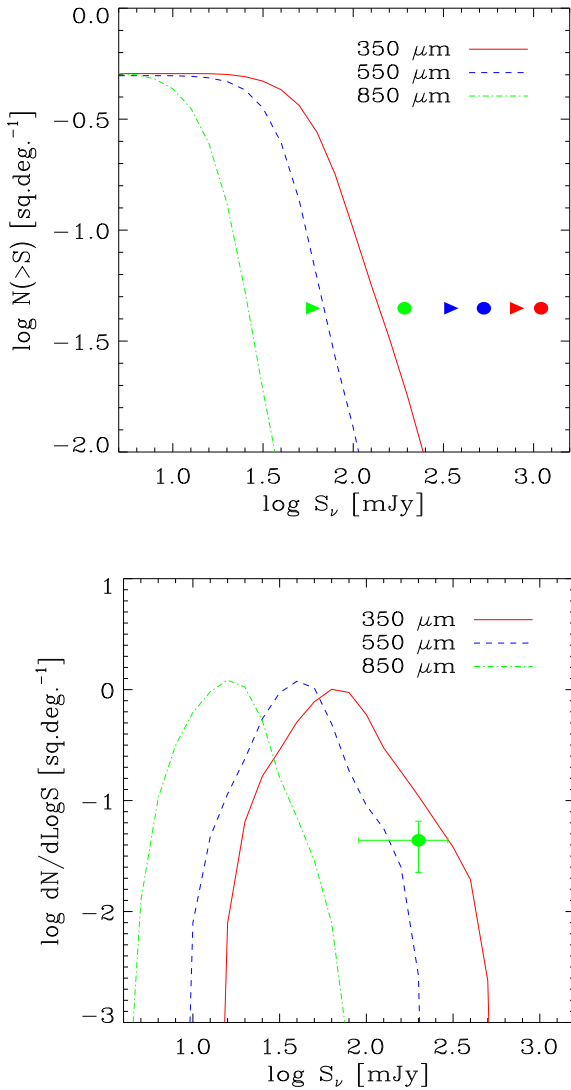
Figure 10. Expected contribution to the cumulative and differential number counts in the Planck HFI bands from the simulated clusters considered in this work, namely all clusters whose final virial mass \gtrsim 1 \times 10^{15} h^{-1} M_\odot , treated as unresolved sources. In the upper panel, the coloured circles (triangles) mark the position corresponding to the average (minimum) fluxes and the number density suggested by the four Planck clumps detected by Clements et al. (2014) over an area of 90 \text{ deg}^2 . In the lower panel, the circle with error bars is the estimate given by these authors at 850 \mu\text{m} .
