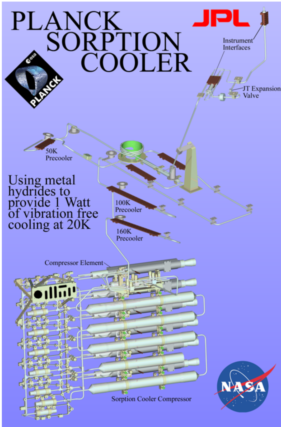
Figure A. Model of flight cooler
