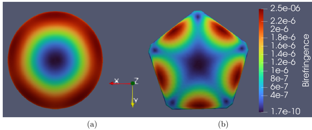
Figure 9. Refractive index difference between the first and second principal directions for the lowermost lens: (a) circular lens, (b) pentagonal lens
