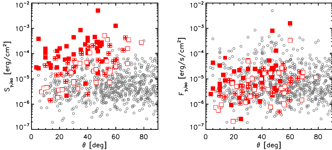
Figure 5. Prompt fluence (left-hand panel) and peak flux (right-hand panel) in the energy range 1\text{--}10^4 keV versus the angle \theta to the LAT boresight. Grey dots represent Fermi GRBs detected only by the GBM. Square symbols represent GRBs detected also by the LAT: filled symbols refer to those with temporally extended emission, empty symbols refer to those with no evidence for extended emission, and empty symbols with a cross inside refer to cases for which the classification is uncertain.
