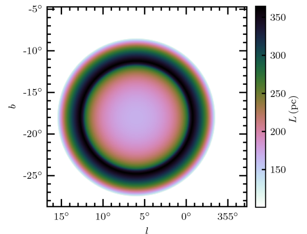
Figure A2. A map of the path-length ( L ) through GSH 006 – 15 + 7, as modelled by equation (A4) and (A5). Here, we adopt a distance to the shell of d_c = 1.5 kpc. The inner and outer radii ( R_i, R_o ) were chosen to match the inner outer bounds of the shell as projected on the sky. These have radii of 6.4 deg and 9.6 deg, respectively.
