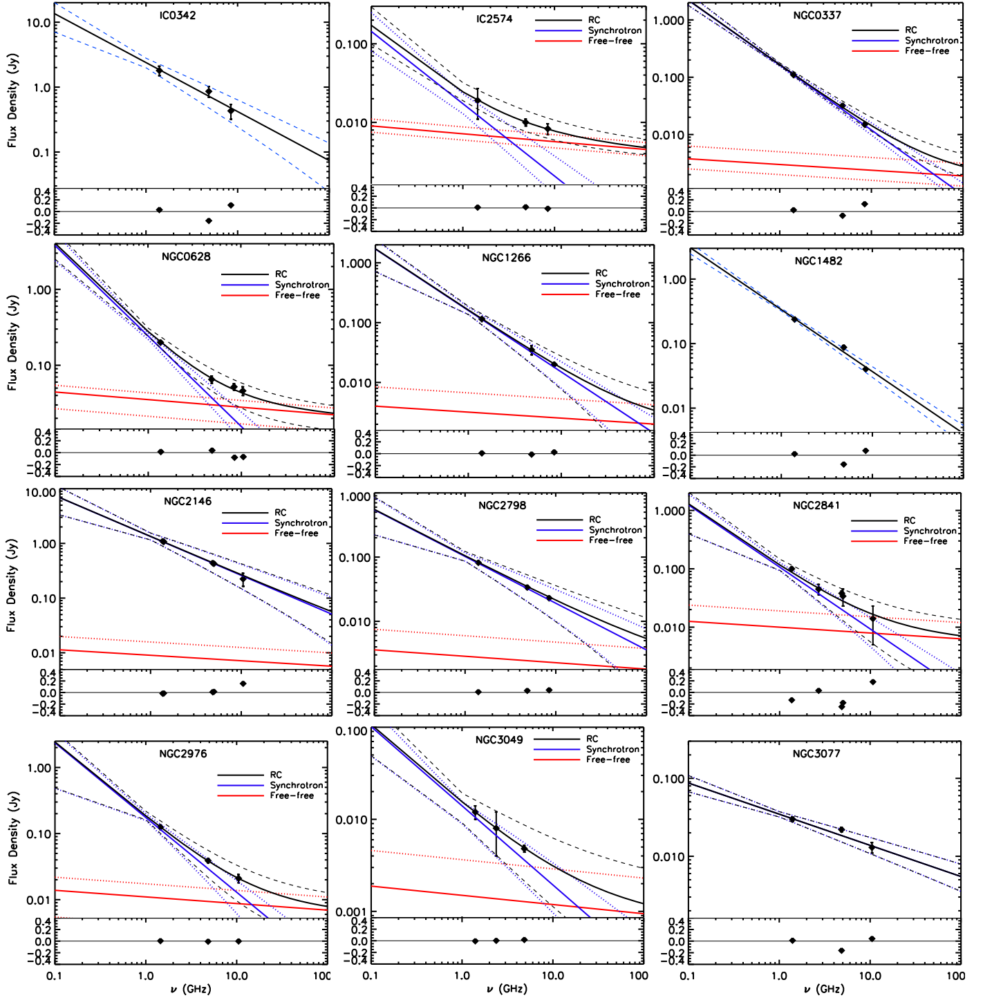
Figure 12. Radio SEDs (flux density vs. frequency) of the KINGFISHER sample (solid curves) for the total RC (black) and its nonthermal (blue) and thermal (red) components as well as their uncertainty curves (dashed for RC and dotted for its components). The points show the observed flux densities. Also shown are the relative residuals (modeled-observed/observed ratio) for each galaxy.
