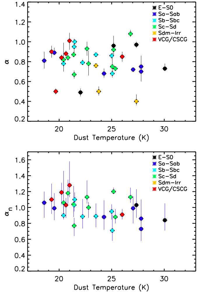
Figure 11. Top: the RC spectral index \alpha vs. the dust temperature. Bottom: the nonthermal spectral index \alpha_{\text{nt}} exhibits a possible decreasing trend against the dust temperature excluding the flat radio sources ( \alpha < 0.6 ).
