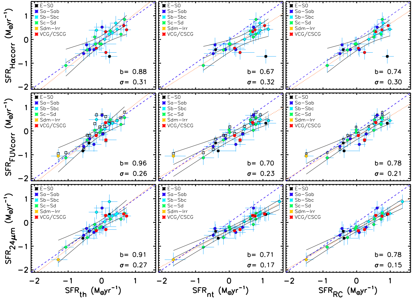
Figure 5. Comparison of the extinction-corrected SFR diagnostics, H\alpha + 24 \mu m ( H\alpha_{corr} ), FUV + 24 \mu m ( FUV_{corr} ), and 24 \mu m plotted from left to right against the 6 cm radio SFRs (thermal, nonthermal, and total, respectively) in logarithmic scale. The galaxies with failed thermal/nonthermal SED fit are excluded. Also shown are the equality line (dashed), the OLS fit and its 95% confidence bounds (solid line/curves), and the bisector fit (dotted line, see Table 7). Here, the slope b refers to the OLS fit. The squares in the second row show the FUV hybrid SFRs calibrated following Boquien et al. (2016). An uncertainty of 30% is assigned for the non-radio SFRs.
