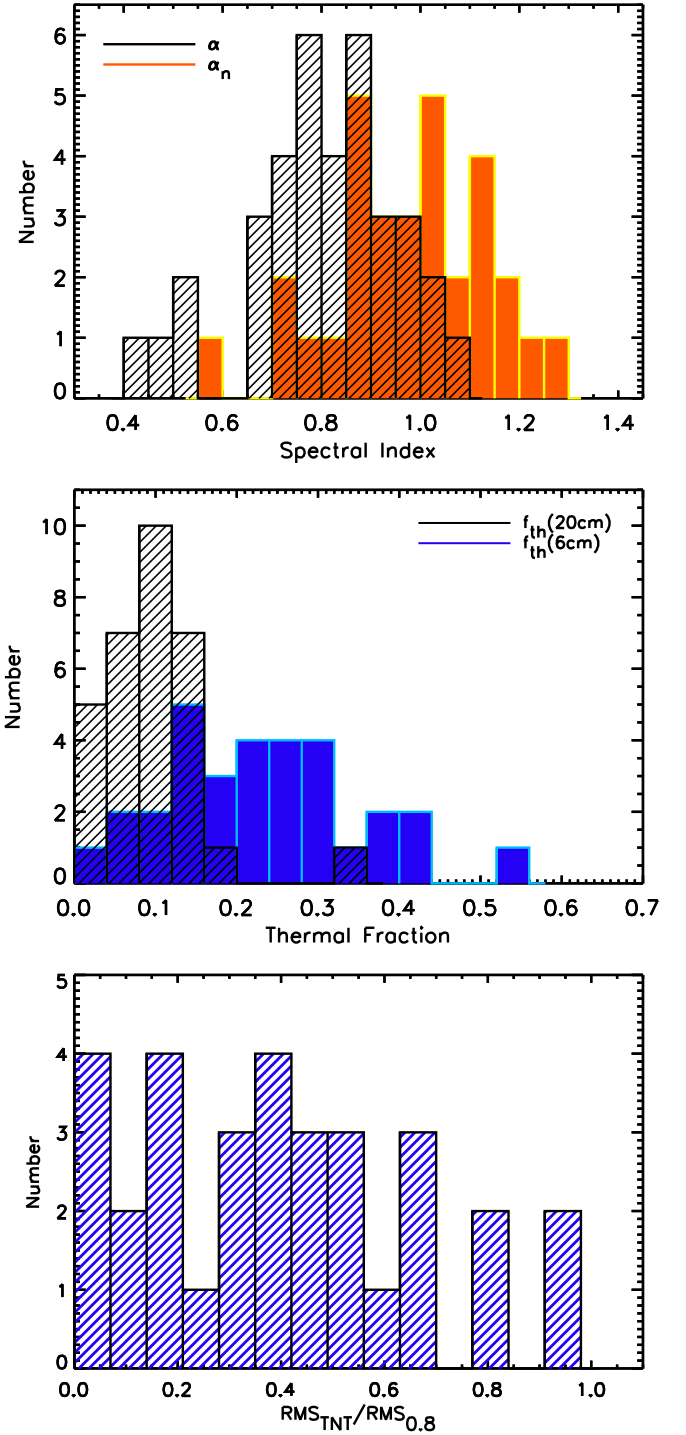
Figure 2. Top: histogram of the spectral index of the total radio continuum emission, \alpha , and its nonthermal component, \alpha_{\text{nt}} , of the KINGFISHER sample. Middle: histogram of the thermal fractions at 6 cm and 20 cm. Bottom: the root-mean-square deviation of the thermal + nonthermal model from the observation, \text{RMS}_{\text{TNT}} , divided by the rms assuming a single power-law model with a fixed spectral index of 0.8 ( \text{rms}_{0.8} ). The first model leads to smaller deviations and hence it is more realistic (the median \text{RMS}_{\text{TNT}}/\text{rms}_{0.8} \simeq 0.4 ).
