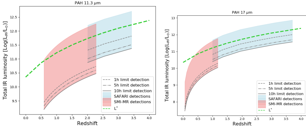
Figure 12. Redshift-luminosity diagrams simulating the SF galaxies detections with SAFARI and SMI MR mode. (a: left:) Detectability of the PAH 11.3 \mu m band. The same color code is applied as in Fig. 10. (b: right:) Detectability of the PAH 17.0 \mu m band.
