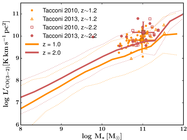
Figure 12. CO J=3-2 luminosity of galaxies as a function of their stellar mass at z = 1 and z = 2 . Observations are taken from Tacconi et al. (2010, 2013). Large squares with the black edges mark the mean CO luminosities at redshift z = 1.2 and z = 2.2 for the combined samples, respectively.
