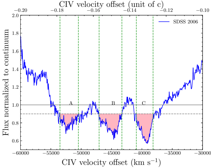
Fig. 5. SDSS 2006 continuum-normalized spectrum of J1538+0855, showing highly blueshifted ( >0.1c ) BAL signatures (A, B, and C) associated with CIV absorption, blueswards of the SiIV emission line. In light pink are indicated absorptions below 90% of the continuum. Green-dashed lines represent the minimum and maximum velocity estimated for the BAL outflow in each trough, respectively. The horizontal dashed line represents the 90% level of the continuum-normalized flux (solid line).
