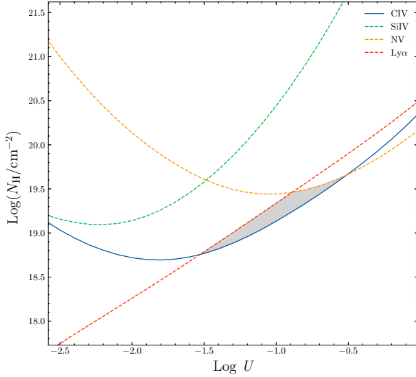
Fig. 9. Theoretical values of U and computed N_H assuming the N_{\text{ion}} lower limit for CIV (solid blue curve), and upper limits for NV (orange-dashed curve), SiIV (green-dashed curve), and Ly \alpha (red-dashed curve) ions for the A component of the UFO BAL in the SDSS 2012 spectrum of J1548+0855.
