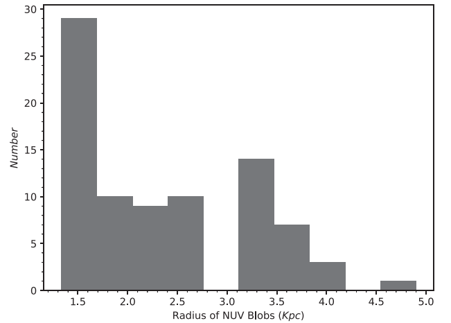
Figure 8. The histogram of the radius of the star-forming knots detected from the NUV image of JO201. The spatial resolution for the NUV image of JO201 is 1.3 kpc.
