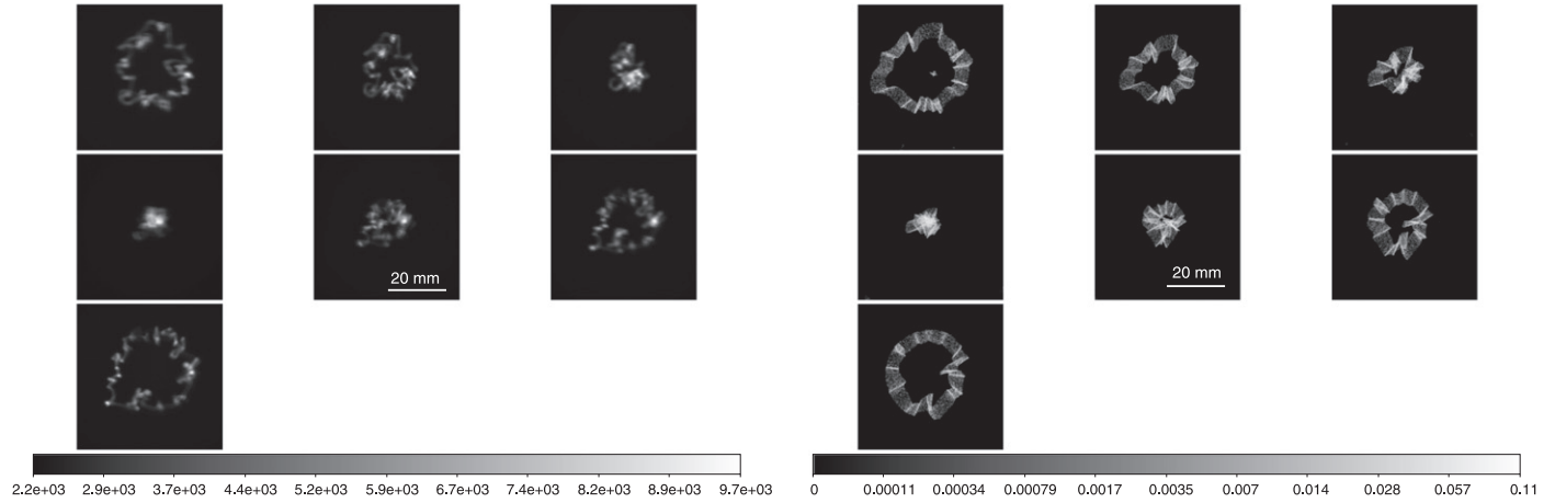
Figure 14. Left: focal series of the measured PSFs for spatial mask 6. From left top extra-focus to bottom right intra-focus PSFs (focus step 5 mm). Right: focal series of the simulated PSFs by Zernike polynomials. There are some discrepancies in the best focus position of the focal series that are visible both from the different PSFs topology and from the different minima position of the focal series in Figure 12.
