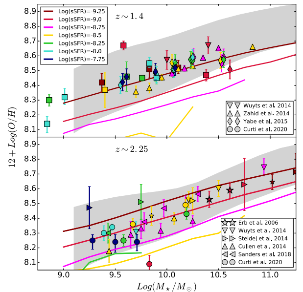
Figure 7. Gas-phase MZR at 1.4 < z < 2.25 . In the left-hand (right-hand) panel, both data and model predictions have been split in colour according to their SFR (sSFR) levels, as indicated in the legend. The grey shaded area shows the predicted MZR as in Fig. 1. Only data with SFR (sSFR) inside the considered model range are shown.
