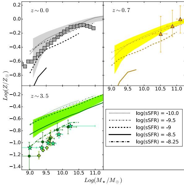
Figure 6. Stellar (left-hand panels) and gas-phase (right-hand panels) MZR s for samples of galaxies at a given sSFR level (as indicated in the legend). All other data points and shaded areas as in Fig. 1.
