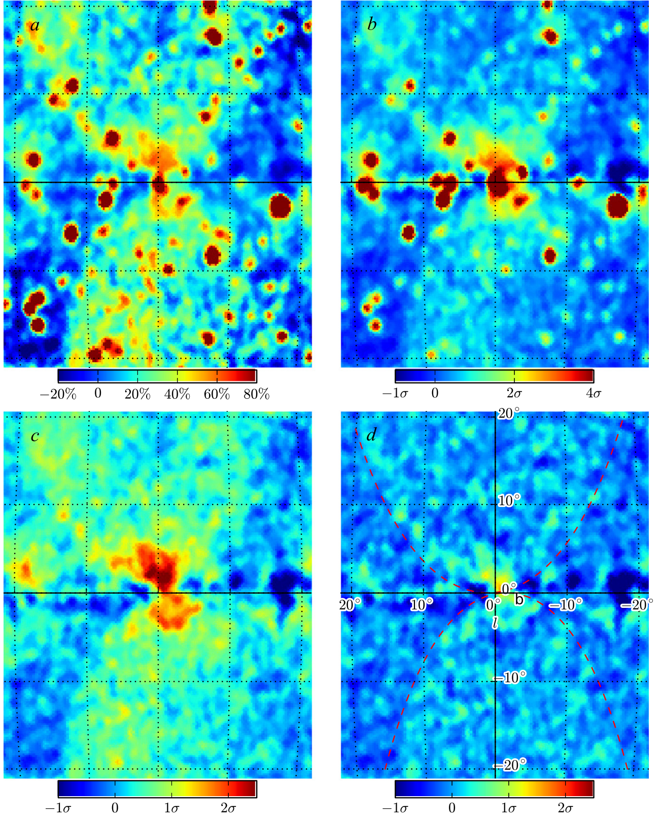
Figure 11. Close-up view of a region within 20° of the GC showing the Fermi -LAT count maps integrated between 1.7 GeV and 50 GeV after subtracting the baseline interstellar model described in Section 7, excluding (top row) and including (bottom row) the point- and extended sources from a preliminary 3FGL list in the model. To reduce the emission contrast in latitude, we display the residuals in fractional units (a), dividing the residuals by the model, and in units of standard deviation (b), dividing the residuals by the square root of the model. In (d) we show the residual map after the further subtraction of I_{\text{EEE}} ; it contains structures smaller than the angular scale included I_{\text{EEE}} . The red dashed lines correspond to the catenary functions that reproduce approximately the edge of the Fermi bubbles for latitudes below 20° (see text for details). We have smoothed the four maps with a Gaussian of 1° FWHM.
