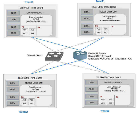
Fig. 9. AXI Trenz-based prototype.
