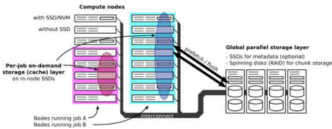
Fig. 4. BeeGFS extended into a two-tier architecture.
