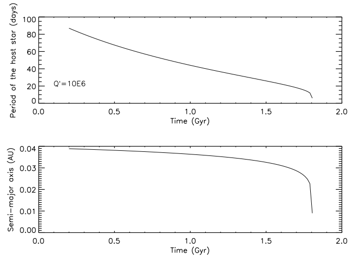
Fig. 7. As Fig. 6, but for Q' = 10^6 .
