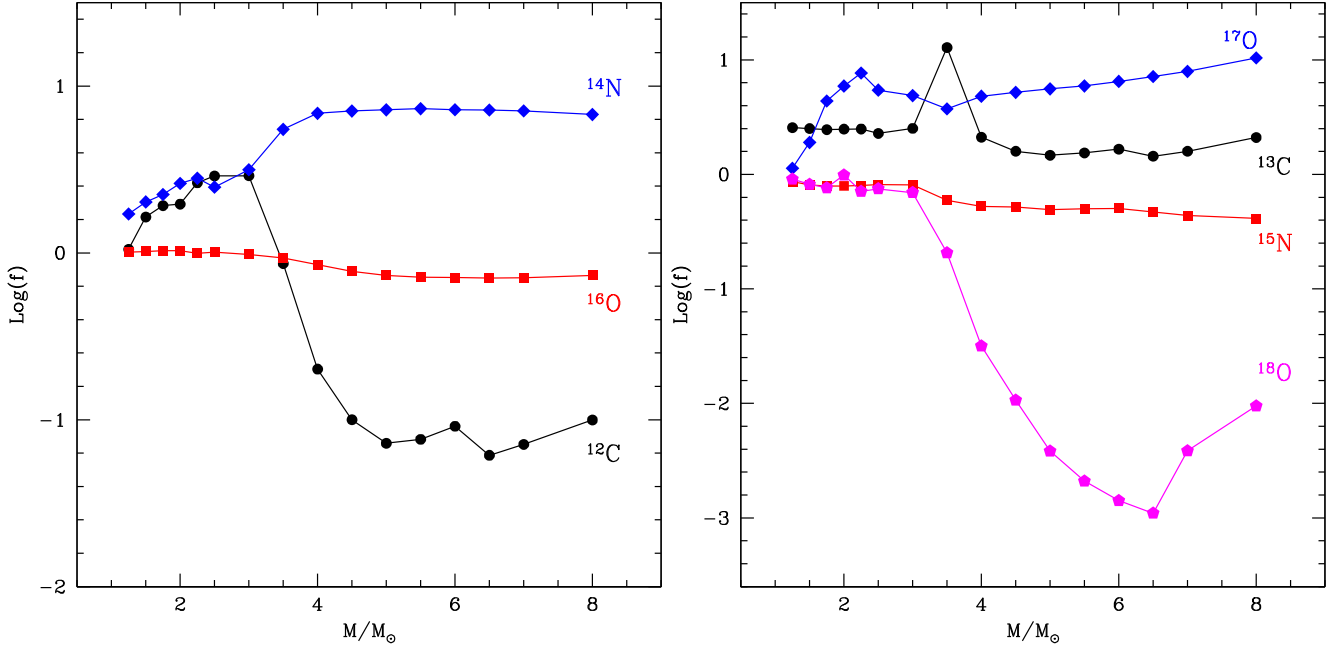
Figure 8. The production factor (see the text for definition) of the CNO isotopes in solar metallicity models. In the left-hand panel, we show the most abundant species, namely ^{12}\text{C} (black points), ^{14}\text{N} (blue diamonds) and ^{16}\text{O} (red squares). The right-hand panel refers to ^{13}\text{C} (black points), ^{15}\text{N} (red squares), ^{17}\text{O} (blue diamonds) and ^{18}\text{O} (magenta pentagons).
