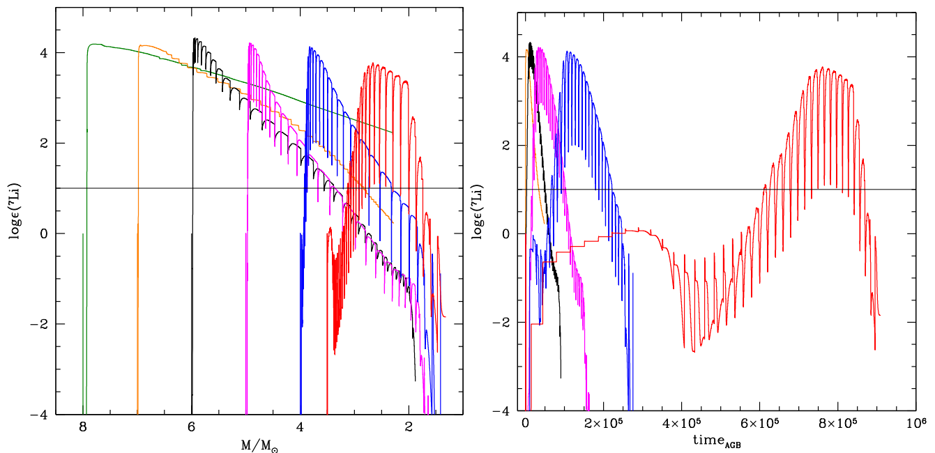
Figure 5. Surface lithium abundance evolution for the same models shown in Fig. 2; the same colour coding is adopted. The quantity on the ordinate is \log(\epsilon(^7\text{Li})) = \log(^7\text{Li}/\text{H}) + 12 . In the left-hand panel, we show the surface lithium as a function of the initial mass, whereas on the right we use the AGB time as abscissa. The horizontal line at \log(\epsilon(^7\text{Li})) = 1 indicates the limit above which the stars are considered lithium-rich.
