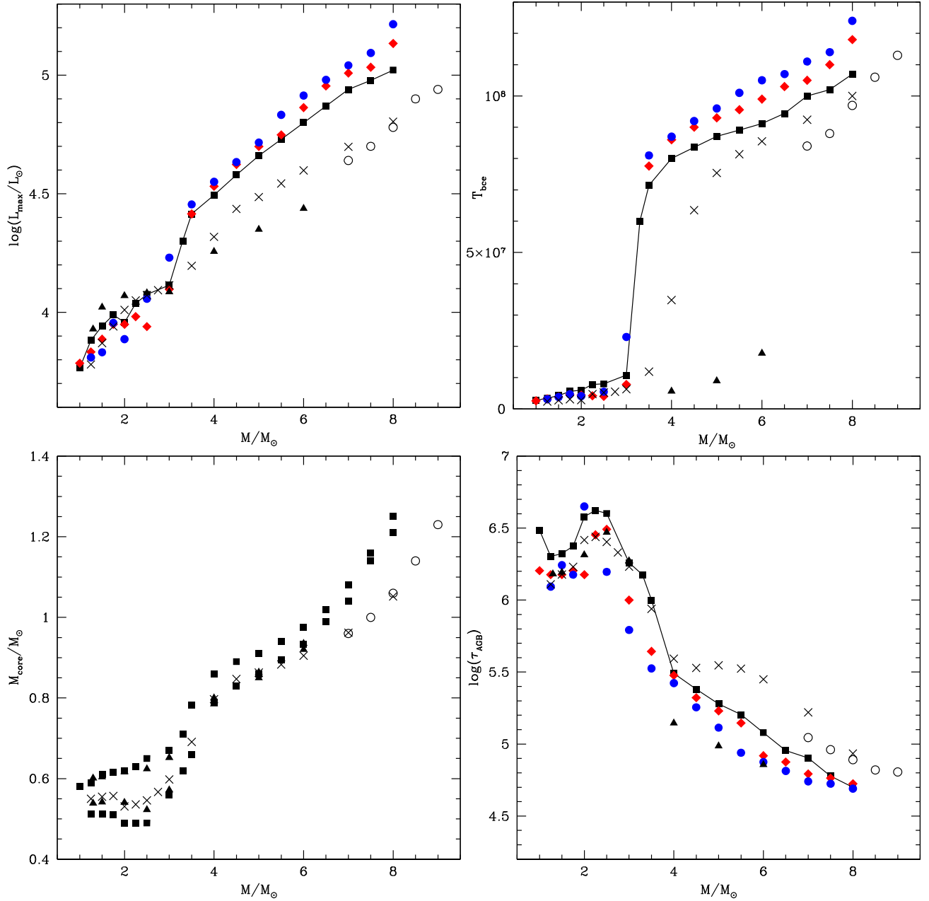
Figure 1. Solar metallicity AGB model properties for various initial masses (filled squares) are presented here. The individual panels show the maximum luminosity reached (top left), the highest temperature experienced at the base of the external mantle (top right), the duration of the TP-AGB phase (bottom right) and the core masses at the beginning and at the end of the AGB evolution (bottom left). The models at Z = 4 \times 10^{-3} and 8 \times 10^{-3} metallicities are indicated, respectively, with blue filled circles and red diamonds. For comparison, we also show the results from Cristallo et al. (2009, 2015, triangles), Karakas & Lugaro (2016, crosses) and Doherty et al. (2014, open circles).
