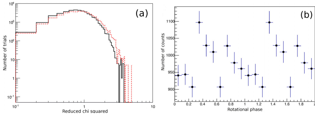
Figure 5. (a) \chi^2/\text{n df} distribution for positions, independent frequencies and frequency derivatives tested in a range of 3\sigma around the expected \nu and \dot{\nu} and of 1\sigma around the central estimate of the coordinates. The black distribution shows the results when using the correct ephemeris whereas the red one refers to the fake ones. (b) Phaseogram obtained by folding the arrival time of the gamma-ray photons with \nu_0 and \dot{\nu}_0 and on the position \lambda_0 and \beta_0 , which results in a maximum in the two periodicity tests applied. Two cycles are plotted for clarity, and the y-axis is zero-suppressed.
