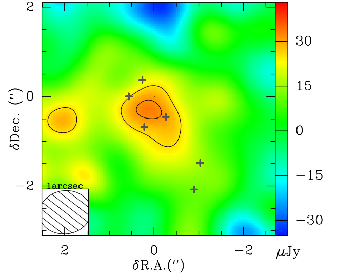
Figure 10. Image of the line-free, 1300 \mu\text{m} continuum of UDF6462 tapered to a 1'' resolution. Contours denote the [2, 2.5] \times noise levels. Grey crosses highlight the position of the clumps identified in Fig. 1.
