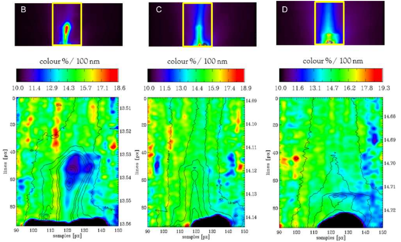
Figure 10. Images of the outburst of September 13 sequence in the VIS at 0.55\ \mu\text{m} (upper plots), and the VIS spatial distribution of the colour (lower plots) calculated in the yellow square of the dust image. The outburst ejecta B and D display colours bluer than the background coma. However, such variations are not seen in outburst C.
