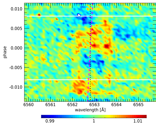
Fig. 12: 2D tomography of H \alpha in the stellar restframe. The vertical dotted line shows the stellar restframe. The diagonal magenta dashed line shows the expected planetary restframe. The horizontal white lines mark the beginning and end of the transit.
