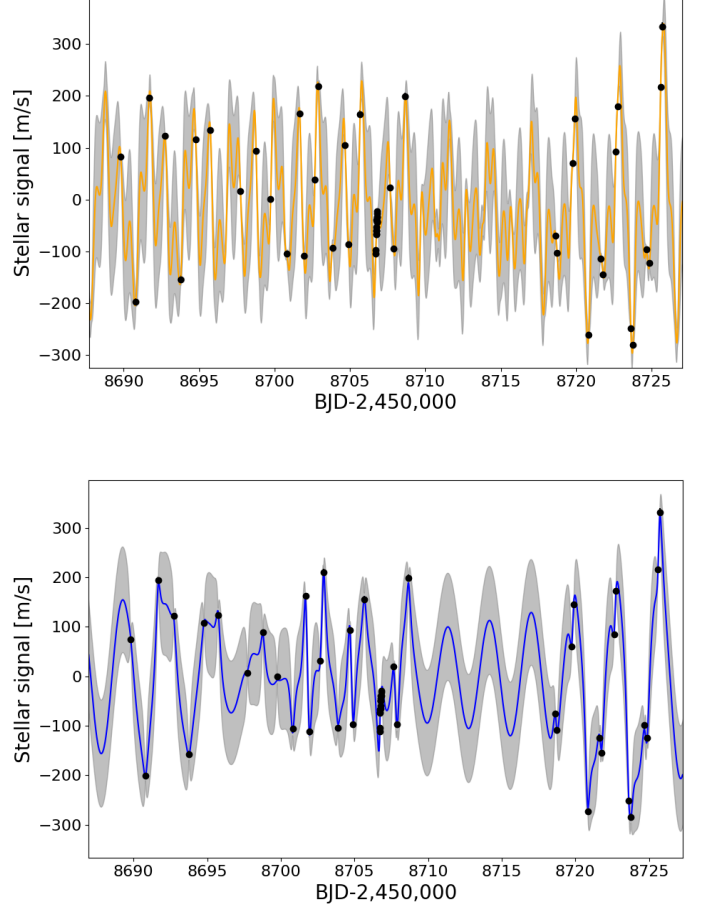
Fig. 6: Upper panel. GP quasi-periodic best-fit model (orange line), as obtained from the joint analysis of the HARPS+ESPRESSO RVs. Here we show a portion of the HARPS time series, after removing the best-fit signal induced by planet b. The shaded area in gray represents the \pm 1\sigma confidence interval. Lower panel. Same as above, but for the GP rotation kernel (blue line).
