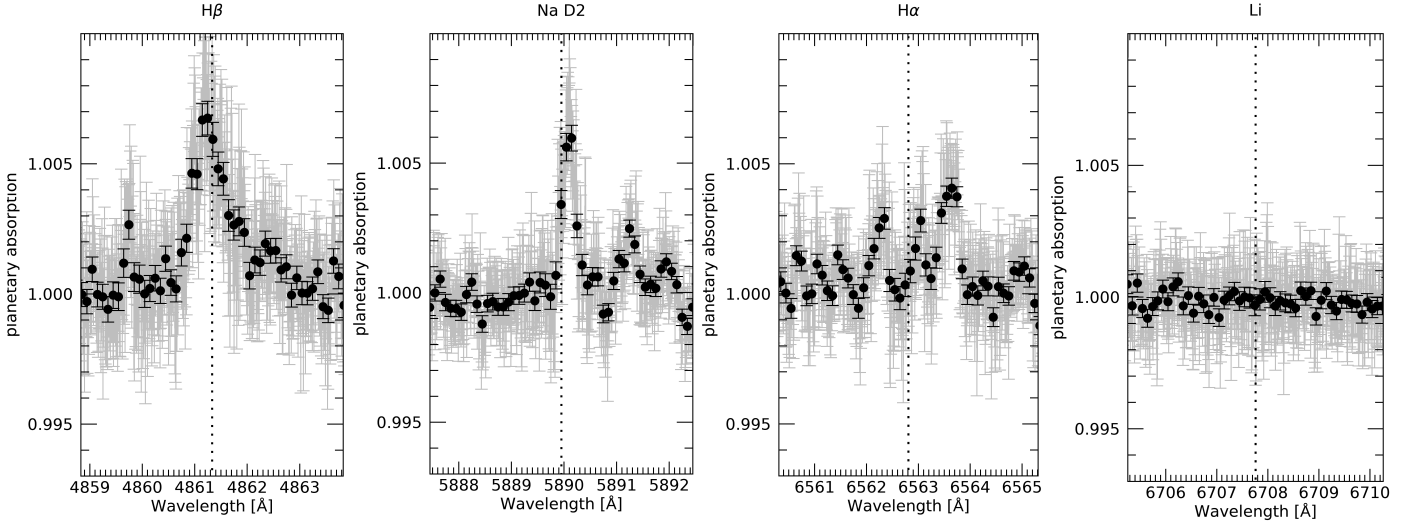
Fig. 13: Transmission spectrum extracted in the zone of the H \beta (left panel), Na D2 (central left panel), H \alpha (central right panel) and Li (right panel) lines. The vertical dashed lines show the planetary restframe. Black points refer to 0.1 Angstrom binning. Different lines we searched for are affected by the contamination given by the stellar activity in different ways.
