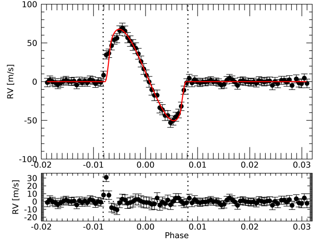
Fig. 10: Upper panel: RM effect for DS Tuc A b from ESPRESSO data modelled by our fit (red line). Vertical dotted lines indicate the transit ingress and egress. Lower panel: Corresponding residuals.
