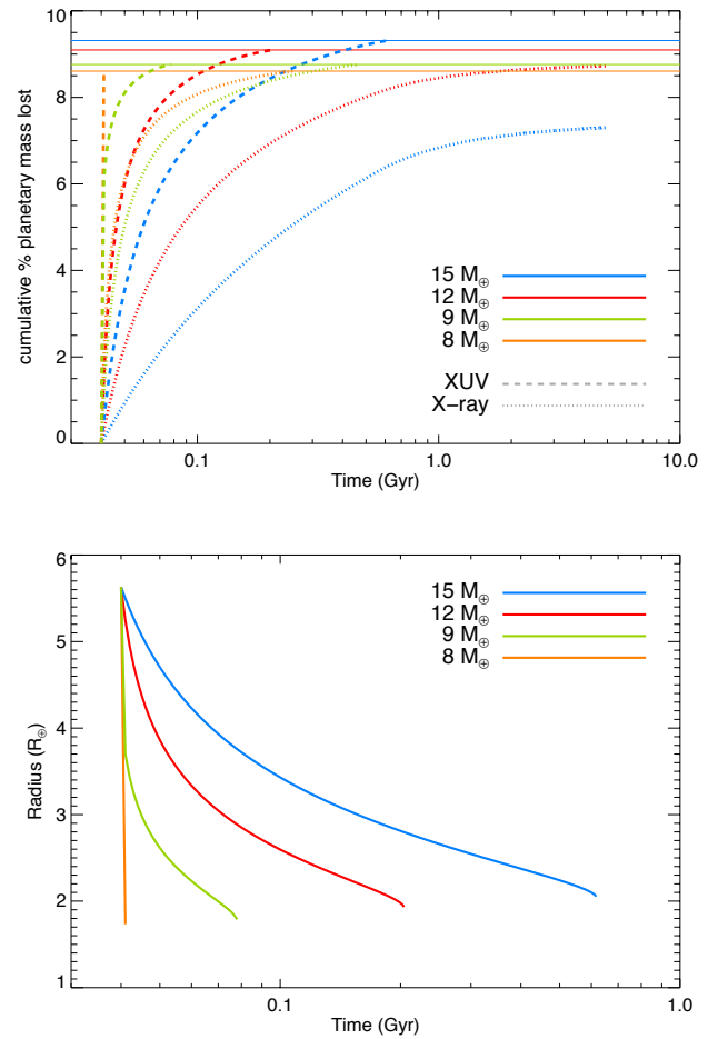
Fig. 17: Upper panel: cumulative percentage of the planetary mass loss evolution considering the X+EUUV irradiation (dashed) or X-ray irradiation alone (dotted). We used the results obtained with the evolution by Penz et al. (2008). Horizontal solid lines represent the limits of the atmospheric mass concerning four representative cases with different starting masses, colour-coded as in the legend. Lower panel: Radius evolution corresponding to the representative cases according to our models from the present age of the system to the end of the photo-evaporation phase.
