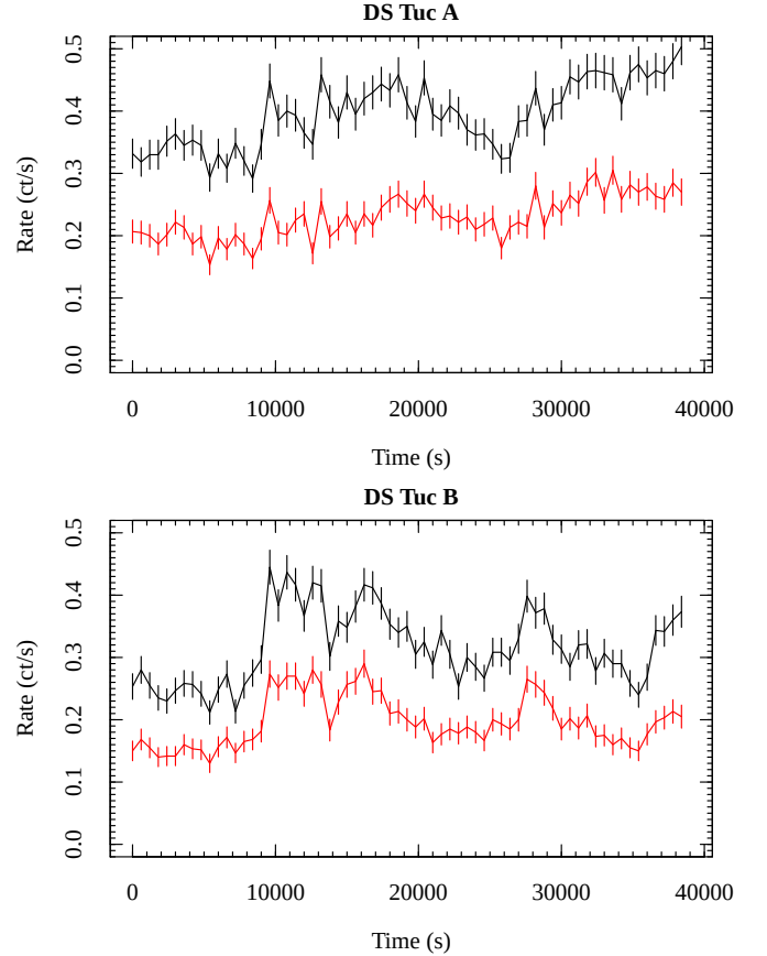
Fig. 15: Top: Mos1 light curves of DS Tuc A. Black line is the light curve from the semi-circular region of radius 30'', red line is the light curve from the circular region of radius 10''. Error bars on rates are at 68% confidence level. Bottom: same for DS Tuc B.
