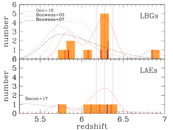
Fig. 5. Upper panel: redshift distribution of all spectroscopically confirmed LBGs at z \sim 6 in the J1030 field. The orange and red histogram have bins of \Delta z = 0.1 and 0.005, respectively. The dashed red curve has been obtained by smoothing the unbinned distribution with a Gaussian with \sigma_z = 0.1 (arbitrarily normalized). The redshift peak and \Delta z \pm 0.1 interval used to estimate the structure significance are shown by the brown vertical dotted lines. The three gray lines show the selection function of i -band dropout samples in the literature (see labels) with selection criteria similar to ours. Lower panel: same as the upper panel but for LAEs selected with MUSE. The gray curve is obtained by heavily smoothing the redshift distribution of LAEs observed with MUSE in the HUDF (Bacon et al. 2017). The QSO redshift (marked in blue) is included in the orange histograms in both panels.
