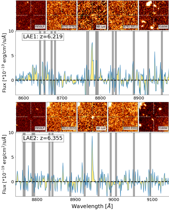
Fig. 3. MUSE spectra of the two LAEs in the LSS (see Table 1) are displayed in two panels. In each panel, the top row shows, from left to right , the HST/ACS F850LP image, three MUSE reconstructed narrow-band images (20 Å-wide), and the HST/Wide Field Camera 3 (WFC3) F160W image. The images are 10'' wide and the source position is indicated by cross-hairs. In the bottom row , the extracted 1D spectrum is shown in a 400 Å-wide interval around the Ly \alpha line, with noisy regions in the MUSE cube affected by the sky line subtraction highlighted by gray bands.
