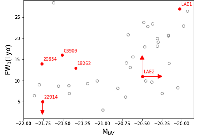
Fig. 4. EW(Ly\alpha) vs. M_{UV} for the six LSS-member galaxies of Table 1 (red filled circle). For comparison, we also plot the same properties from a large sample of high- z galaxies, presented by De Barros et al. (2017; gray empty circles).
