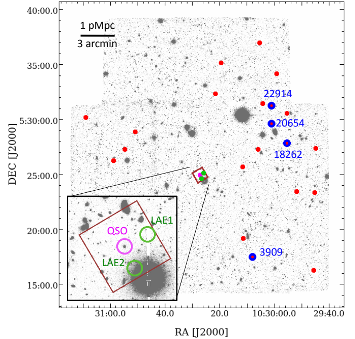
Fig. 1. Sky distribution of the LBG sample (red dots) overplotted to the LBT/LBC z -band image of the field. The spectroscopically confirmed members of the LSS at the QSO redshift are marked in blue and labeled with their ID. The position of the two LAEs in the LSS discovered by MUSE is marked by green points. The MUSE field of view (FOV) is shown as a brown square. The position of the QSO is shown in magenta. The inset shows a zoom on the sky region around the MUSE field.
