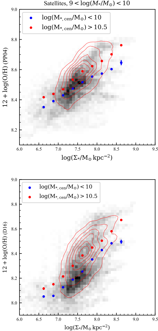
Figure 6. The local \Sigma_{*} – O/H relation for satellite galaxies with 9 < \log(M_{*}/M_{\odot}) < 10 split by the mass of the galaxy which is central to their halo. In the upper panel, we show the results for the PP04 indicator, and in the lower panel we show the results for the D16 indicator. Blue points show the median metallicity at a given \Sigma_{*} for satellites of low-mass centrals ( \log(M_{*}/M_{\odot}) < 10 ). These points trace the median of the grey-shaded distribution. Red points are the median metallicity as a function of \Sigma_{*} for satellites of high-mass centrals, shown by the red contours. The oxygen abundance is systematically higher for satellites of more massive centrals.
