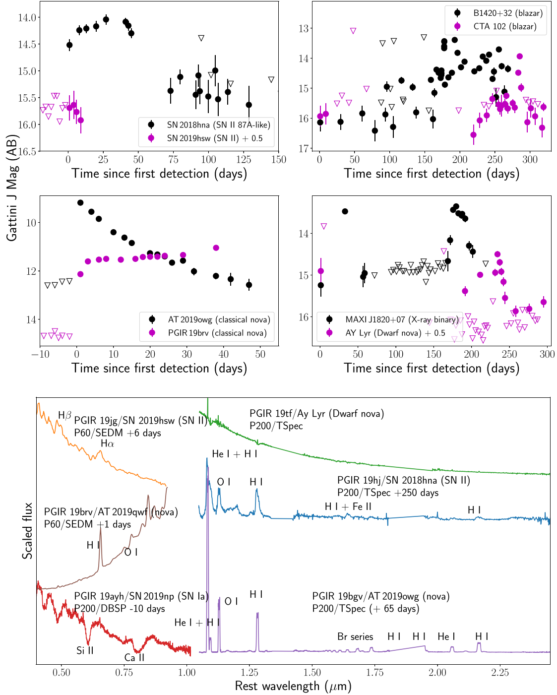
Figure 27. (Top panel) Collage of light curves of extragalactic and Galactic transients detected with Gattini. Circles denote detections while inverted triangles are 5\sigma upper limits. The extragalactic transients include the Type II SN 1987A-like SN 2018hna (PGIR 19hj) and Type II SN 2019hsw (PGIR 19jg), as well as the large amplitude flaring blazars B1420+32 (PGIR 19c) and CTA 102 (PGIR 19ayd). The Galactic transients include the reddened classical novae PGIR 19brv (AT 2019qwf) and PGIR 19bgv (AT 2019owg), a flaring X-ray binary MAXI J1820+07 (PGIR 19auj) and a recurrent dwarf nova Ay Lyr (PGIR 19tf). (Lower panel) Optical and NIR spectra obtained as follow-up for some of these sources, marking the prominent spectral lines in each source. In addition, we show an optical spectrum of the Type Ia SN 2019np (PGIR 19ayh).
