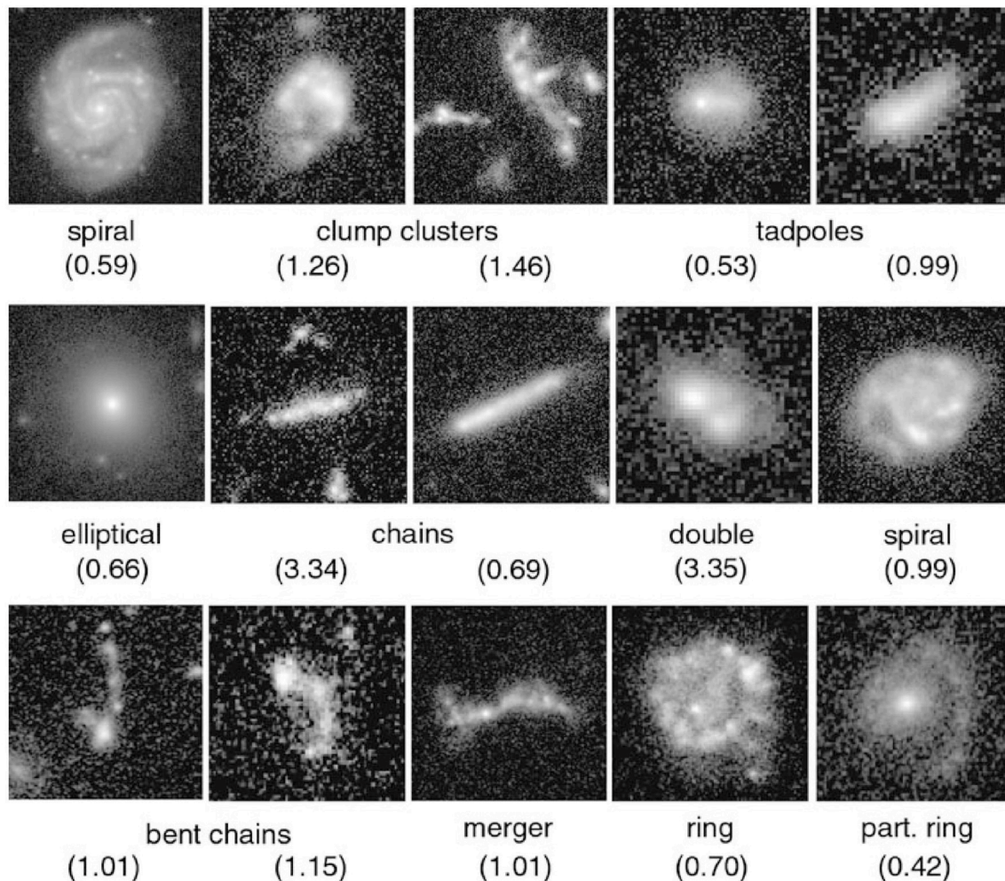
FIGURE 5 | Morphology of galaxies at intermediate and high redshift. Redshift is given by numbers in parentheses. (Credit to Buta, 2013, his Figures 1–46, from Planet and Stellar Systems).
