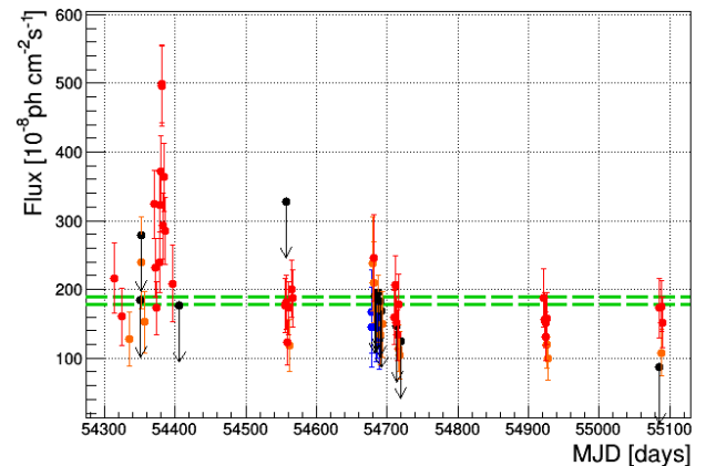
Fig. 16. Light curve of the Crab pulsar+nebula in the energy range 100 MeV–10 GeV, with a one-day resolution. The black downward arrows represent 2\sigma upper limits. The blue, orange, and red circles refer to a \sqrt{TS} \geq 3 , \geq 4 and \geq 5 , respectively. The green dashed lines indicate the average flux plus/minus the error from Table 10.
