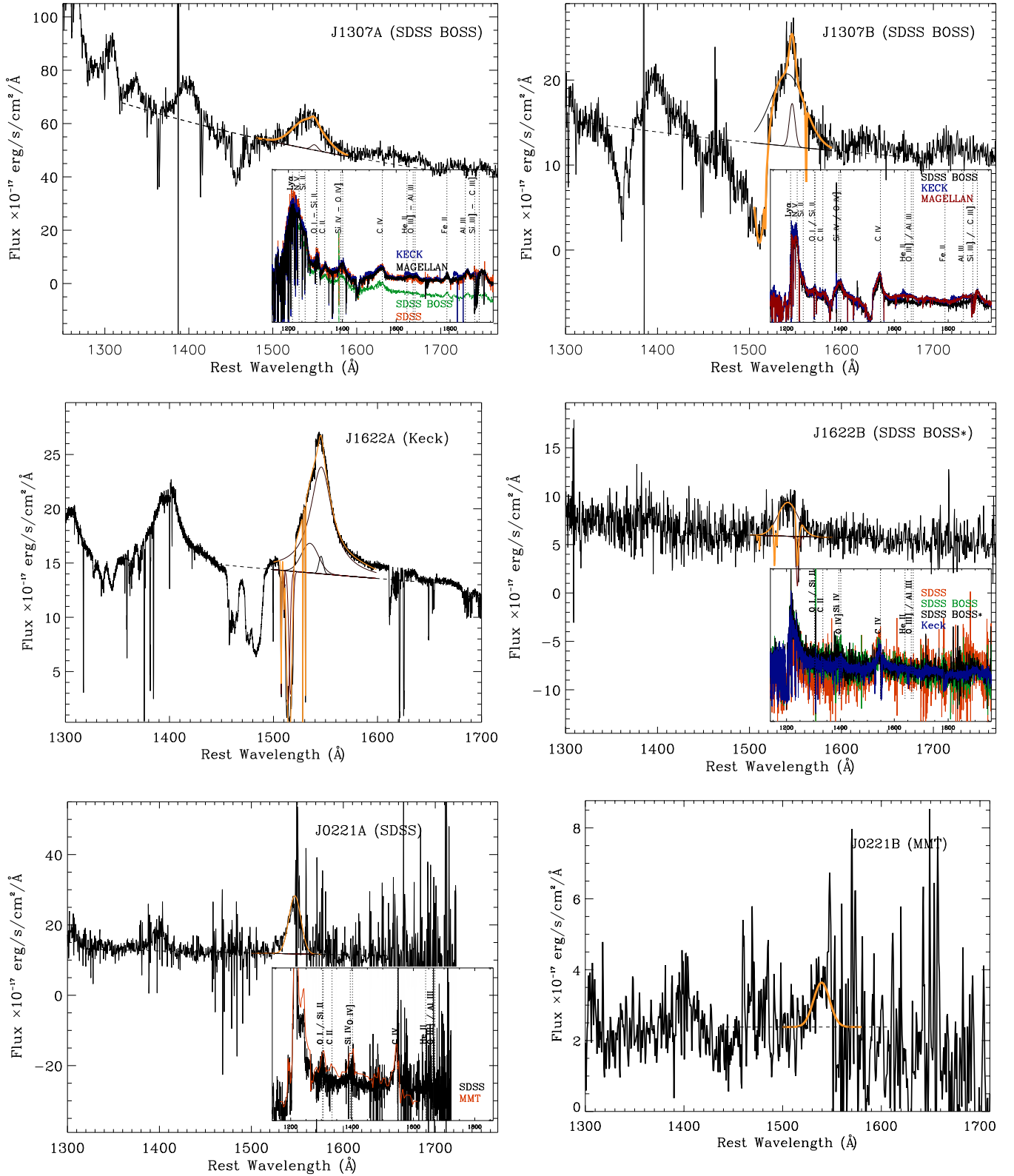
Figure 3. Rest-frame UV spectra of the quasar pairs around the C IV line showing our fitting method. Superimposed on the spectra are the best-fitting components (see § 4): a power law (dashed line), tracing the continuum emission, and Gaussian profiles (black solid curves), reproducing the C IV emission line. The orange solid curve represents the sum of all components, including a set of negative Gaussian profiles which take into account the BAL contribution when needed. In the insets, we show the various spectra of each quasar (when available) collected from archival data, which allowed us to prove the absence of significant luminosity variability, with the exception of J1307A. For J1307A and J1622B, we selected the SDSS BOSS spectra closer to the X-ray observation. For J0221B, the region at wavelength of 1545 Å has been excluded from the fit, because of the strong sky-subtraction residuals affecting the C IV line profile (see Fig. 3 of McGreer et al. 2016). Vertical dotted lines mark the wavelength of UV emission lines in the range 1150–1950 Å.
