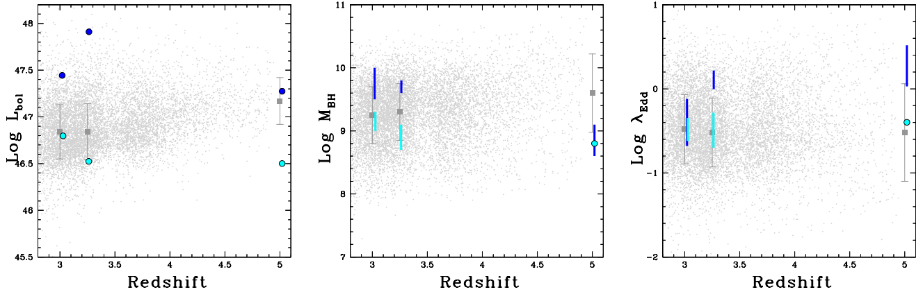
Figure 4. Comparison of the properties of the three quasar pairs of the current work vs. SDSS quasars (from the compilation of Shen et al. 2011b , updated as Nov. 2013, small grey dots): bolometric luminosity vs. redshift (left panel), black hole mass vs. redshift (middle panel) and Eddington ratio vs. redshift (right panel). The grey squares represent the median values from the SDSS quasars in redshift ranges encompassing/close to those of our sources, while the error bars show the 1\text{-}\sigma dispersion. The A (B) quasar components of our sample are shown as blue (cyan) symbols and bars; the black hole mass and Eddington ranges (excluding J0221B) are computed as described in §4, assuming negligible error on the derived bolometric luminosity (see Richards et al. 2011 ).
