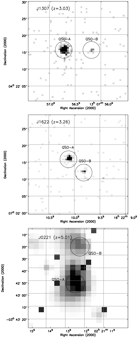
Figure 1. 0.5–7 keV band Chandra images of J1307 (top) and J1622 (middle) quasar fields. Each box side is 30'' ; the circles (diameter= 5'' ) mark the quasars of the pairs. The QSO field of J0221 as observed by XMM- Newton (pn camera, 0.3–3 keV band) is shown in the bottom panel; each side of the box is \approx 85'' , and circles have a diameter of 15'' . All images keep the original pixel size ( \approx 0.5'' for Chandra and \approx 4.1'' for XMM- Newton /pn).
