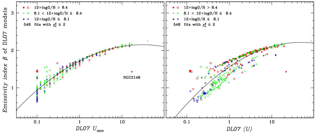
Fig. 15. Best-fit DL07 emissivity index \beta_{\text{DL07}} plotted against U_{\text{min}} (in the left panel) and \langle U \rangle (in the right). Only those MBBV DL07 fits with \chi^2_\nu \leq 2 are considered in the plot. As before, points are coded by oxygen abundance. The curve in the left panel is the second-order polynomial best-fit of DL07 MBBV \beta to \log_{10}(U_{\text{min}}) : \beta_{\text{DL07}} = 1.72 + 0.58 \log(U_{\text{min}}) - 0.20 \log^2(U_{\text{min}}) . The right panel shows the analogous curve for \log_{10}(\langle U \rangle) : \beta_{\text{DL07}} = 1.56 + 0.77 \log(\langle U \rangle) - 0.23 \log^2(\langle U \rangle) .
