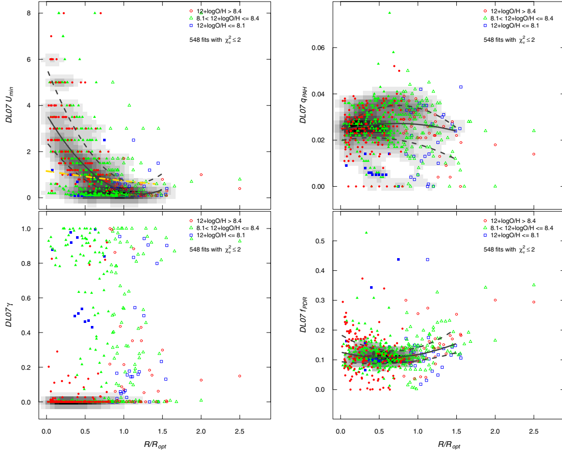
Fig. 11. Best-fit DL07 parameters plotted against normalized galactocentric distance. The upper left panel shows U_{\text{min}} ; the upper right q_{\text{PAH}} ; the lower left \gamma ; and the lower right PDR fraction f_{\text{PDR}} . The underlying grayscales in each panel show the two-dimensional density distributions of the data. The upper left and right panels show the mean (solid curve) and quartiles (dashed curves) of U_{\text{min}} (upper left), q_{\text{PAH}} (upper right) and f_{\text{PDR}} (lower right). The (yellow) long-dashed curve in the upper left panel shows the relation for U_{\text{min}} = U_0 (T_{\text{dust}}/T_0)^{(4+\beta)} for U_0 = 0.93 , T_0 = 22 K, and \beta = 1.8 as described in the text. As in previous figures, (red) circles correspond to 12+\log(\text{O}/\text{H}) > 8.4 , (green) triangles to 8.1 < 12+\log(\text{O}/\text{H}) \leq 8.4 , and (blue) squares to 12+\log(\text{O}/\text{H}) \leq 8.1 ; filled symbols indicate R/R_{\text{opt}} < 0.8 .
