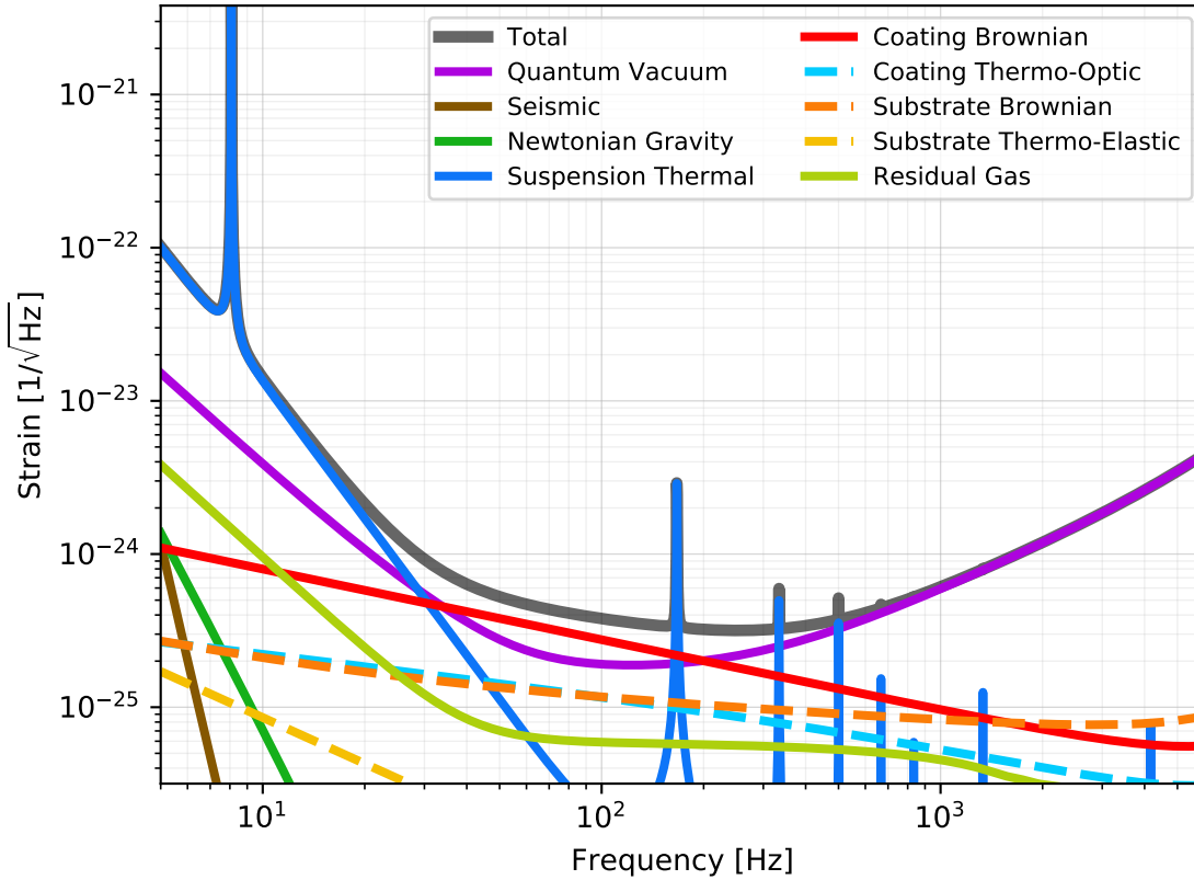
Figure 2. Noise budget for ET-HF assuming 3MW power in the cavities, fused silica mirrors of 200 Kg weight working at room temperature and a laser wavelength of 1064 nm
