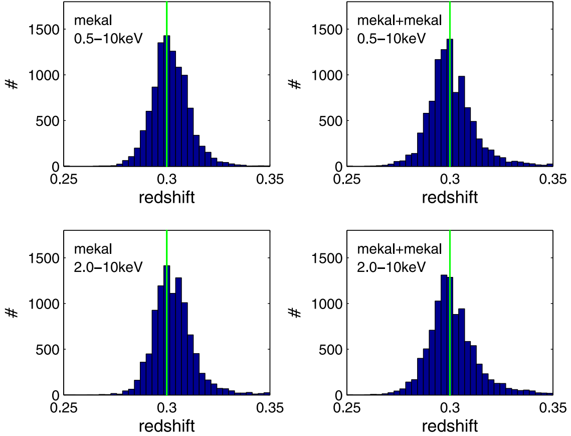
Figure 1. Upper left panel: distribution of the best-fit X-ray redshift z_X obtained fitting with a single-temperature mekal model a total of 10^4 spectra simulated assuming a two-temperature mekal model as an input with kT_1 = 8 keV and kT_2 = 15 keV, Z_1 = 0.6 Z_\odot , Z_2 = 0.4 Z_\odot , and the same emission measure. A third component with kT_3 = 3.5 keV and Z_3 = 1.0 Z_\odot has been added with a 10\times lower emission measure. The redshift z_{\text{input}} = 0.30 (shown as a vertical green line) is the same for both components. Simulated spectra have an average of 2 \times 10^4 net counts in the 0.5–10 keV band. Fits are performed over the entire energy range (0.5–10 keV). Upper right panel: same as the upper left panel, but using a two-temperature mekal model to fit the simulated spectra. Lower left panel: same as the upper left panel, but fitting only the hard band (2.0–10 keV). Lower right panel: same as the upper right panel, but fitting only the hard band (2.0–10 keV).
