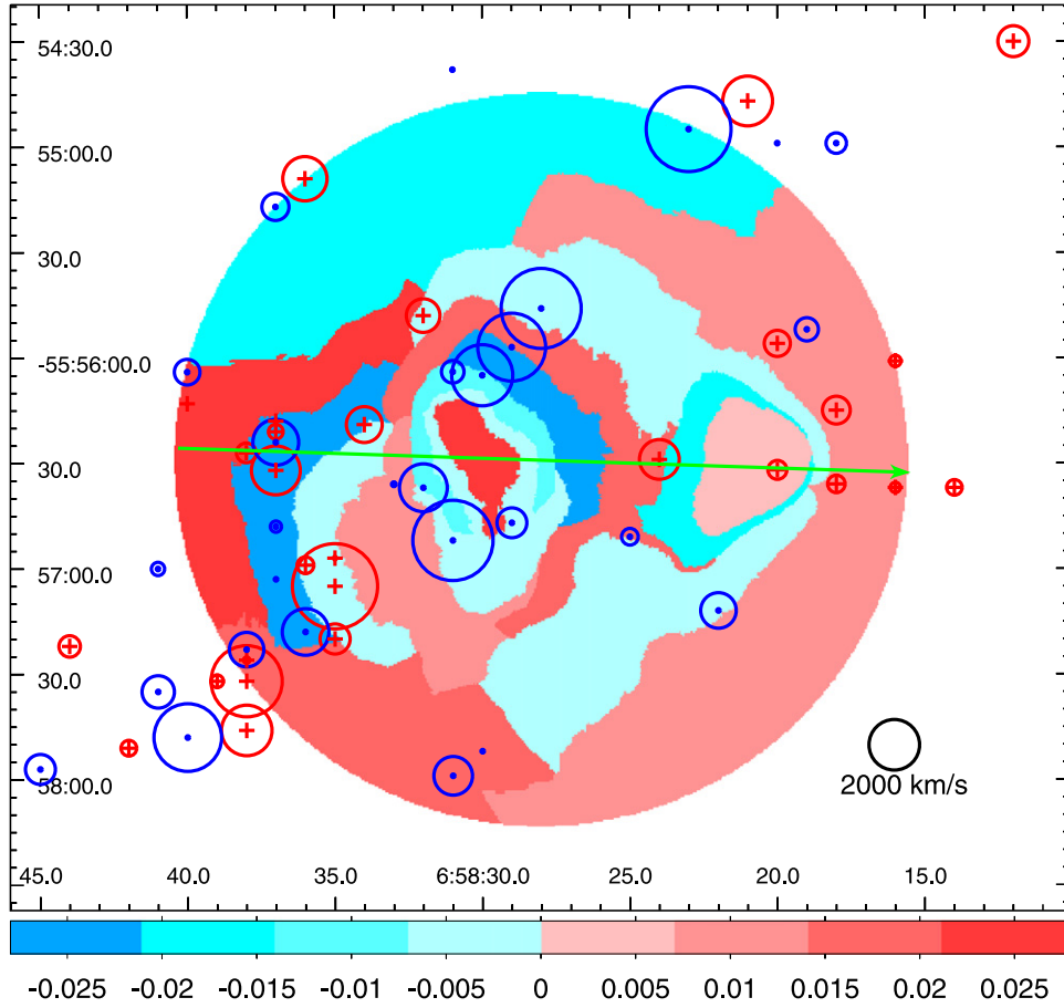
Figure 12. Spatial distribution of 80 member galaxies overplotted on the ICM redshift map. The radius of the circles is proportional to the peculiar velocity of the galaxy. Red circles and red crosses stand for member galaxies with v_{\text{rest}} > 0 , while blue circles and blue dots stand for member galaxies with v_{\text{rest}} < 0 . The green arrow shows the directions we consider to explore the X-ray redshift along the bullet trail (see Figure 13).
