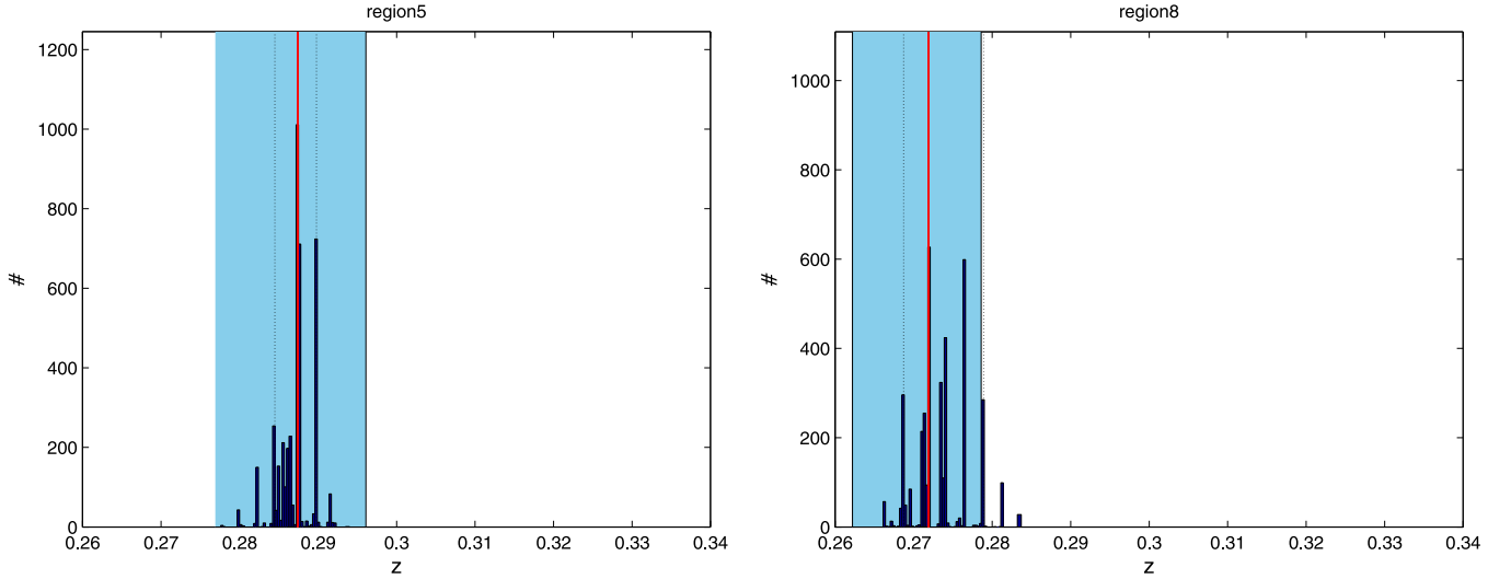
Figure 6. Histogram distribution of best-fit z_X ( T_1 , T_2 , Z_1 , Z_2 ) computed on the subgrid of temperature and abundance values selected as described in the text, for region 5 (left panel) and region 8 (right panel). The central vertical line shows the absolute best-fit z_X , the dashed area shows the range due to the statistical errors on the absolute best-fit z_X , and the two vertical dashed lines the lower and upper 90% percentiles of the z_X ( T_1 , T_2 , Z_1 , Z_2 ) distribution.
