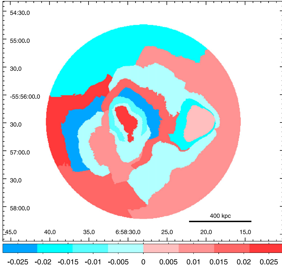
Figure 5. Redshift map of the ICM in the Bullet cluster computed with respect to the average redshift \langle z_X \rangle = 0.2986 . The color bar used discrete steps equal to \Delta z = 0.007 which corresponds approximately to the typical 1\sigma error on z_X .
