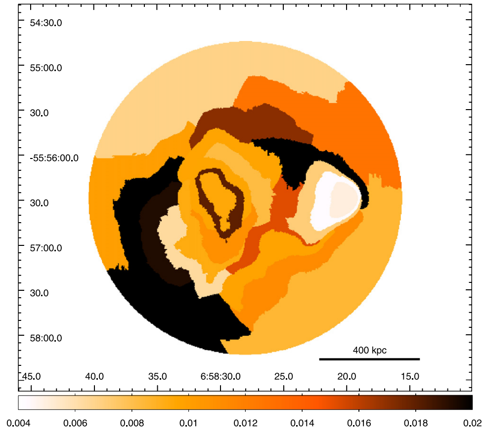
Figure 7. Map of the statistical 1\sigma error on the X-ray redshift z_X .
