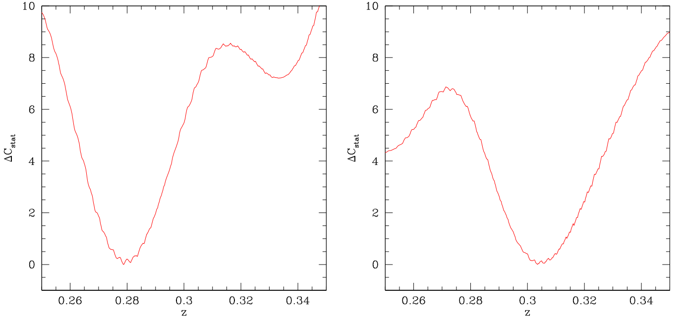
Figure 4. Plot of \Delta C_{\text{stat}} vs. redshift for region 4 (left panel) and region 9 (right panel).
