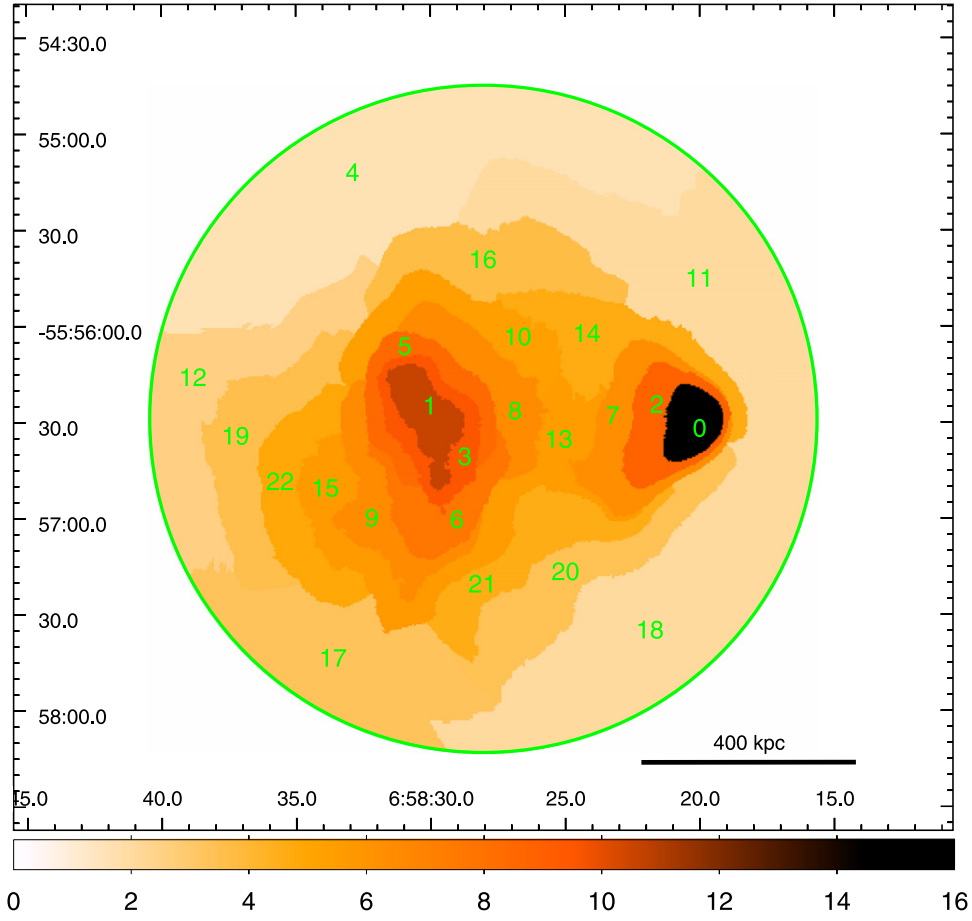
Figure 3. Color-coded surface brightness map of the Bullet clusters. Each of the 23 regions defined by the contour-binning technique are shown with a different color corresponding to the hard-band surface brightness. The units of the color bar are counts per pixel. The large circle shows the region used to extract the spectrum of the global cluster emission.
