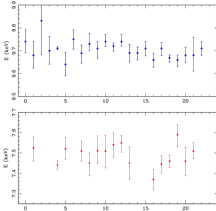
Figure 15. Best-fit energies for the fluorescent lines of Au L_{\alpha} (upper panel) and Ni K_{\alpha} (lower panel) lines in each region with the corresponding 1\sigma error bars. Note that we are not able to identify the Ni K_{\alpha} line in several regions, while the Au L_{\alpha} line is always detected.
