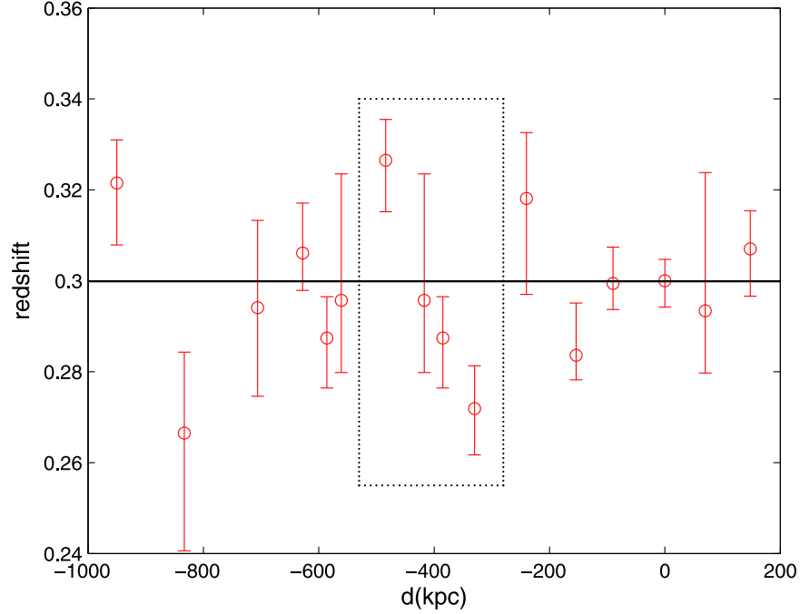
Figure 13. Redshift measured along the direction of the bullet where the x -axis is the distance from the peak of the X-ray brightness (the head of the bullet). The average redshift \langle z_x \rangle = 0.2986 is shown as a horizontal line. The dashed box roughly identifies the region in which we observe a velocity gradient of (46 \pm 13) \text{ km s}^{-1} \text{ kpc}^{-1} .
