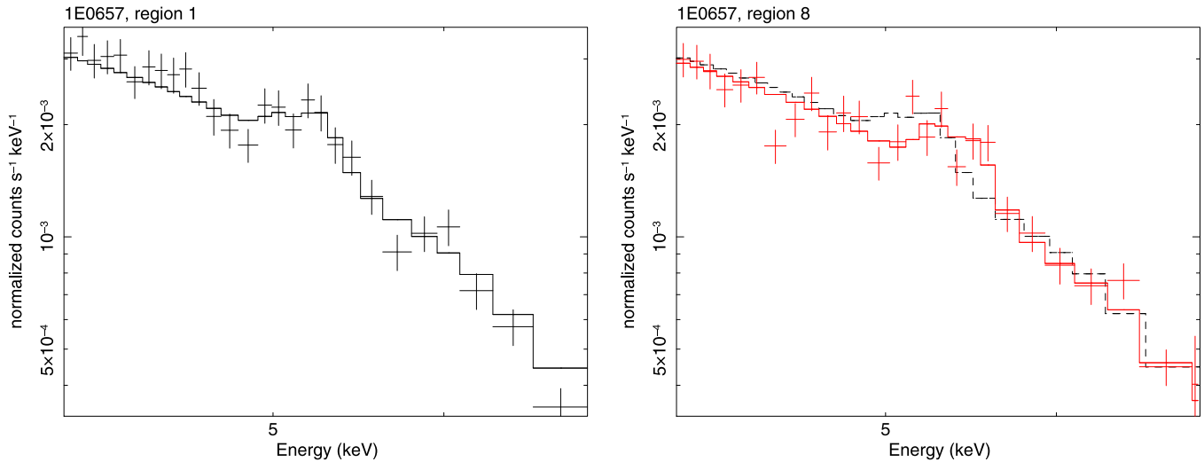
Figure 10. Folded spectra of the two regions with the most extreme redshift (left panel: region 1; right panel: region 8). The spectra are binned to a minimum of S/N = 9 , and only the 4.0–7.0 keV energy range is shown. The solid lines show the best-fit model obtained fitting the 2.0–10 keV energy band with two mekal components. The dashed line in the right panel shows the best-fit model of region 1.
