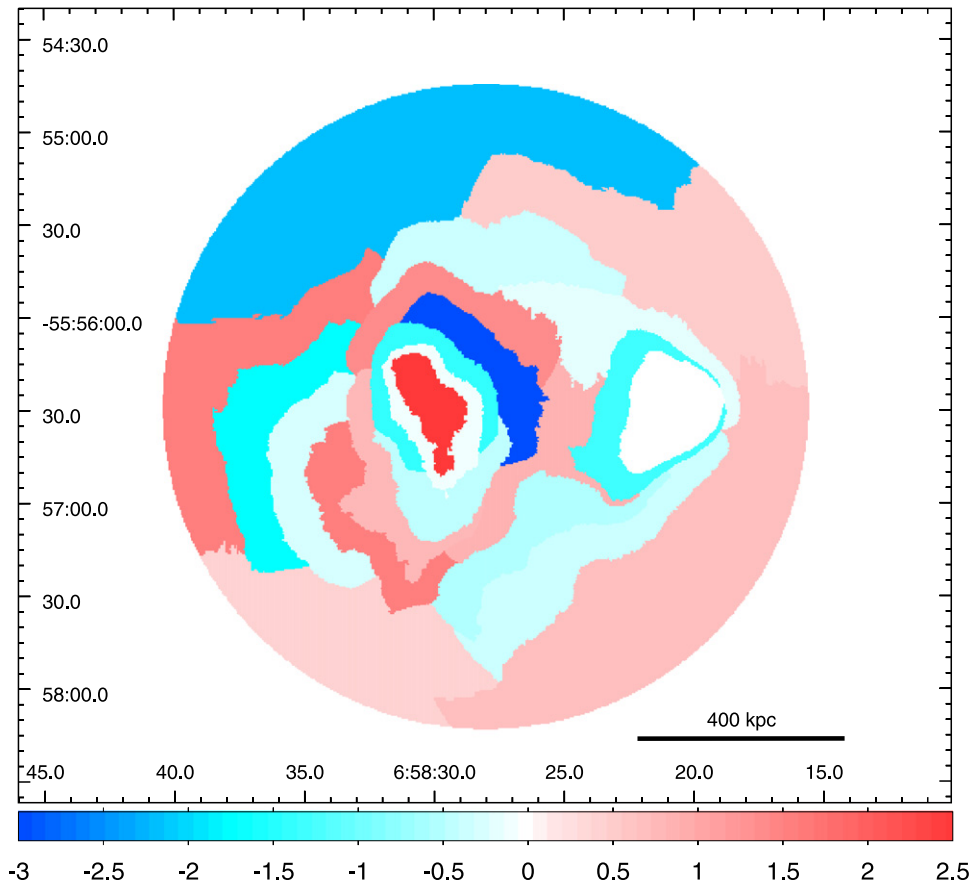
Figure 9. Significance map obtained as (z_X - z_{\text{avg}})/\sigma_{\text{tot}} . Only two symmetric regions stand out in bright red and blue colors, while all of the remaining regions have z_X within less than 2\sigma from \langle z_X \rangle .
