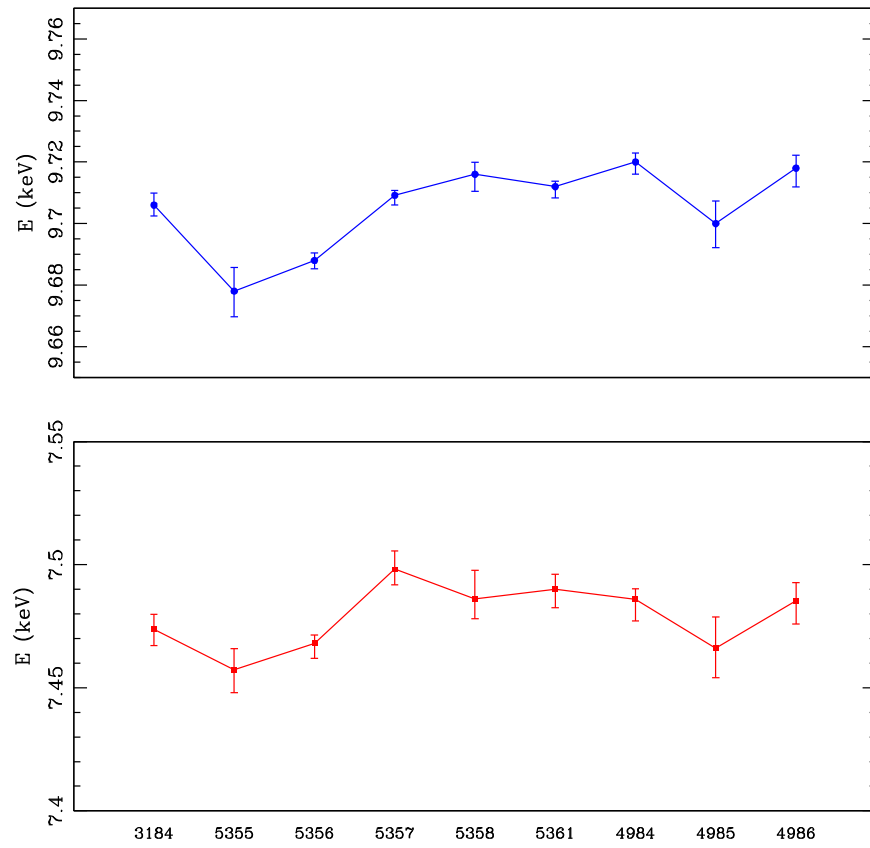
Figure 14. Best-fit energies for the fluorescent lines of Au L_{\alpha} (upper panel) and Ni K_{\alpha} (lower panel) in each Obsid with corresponding 1\sigma error bars.
