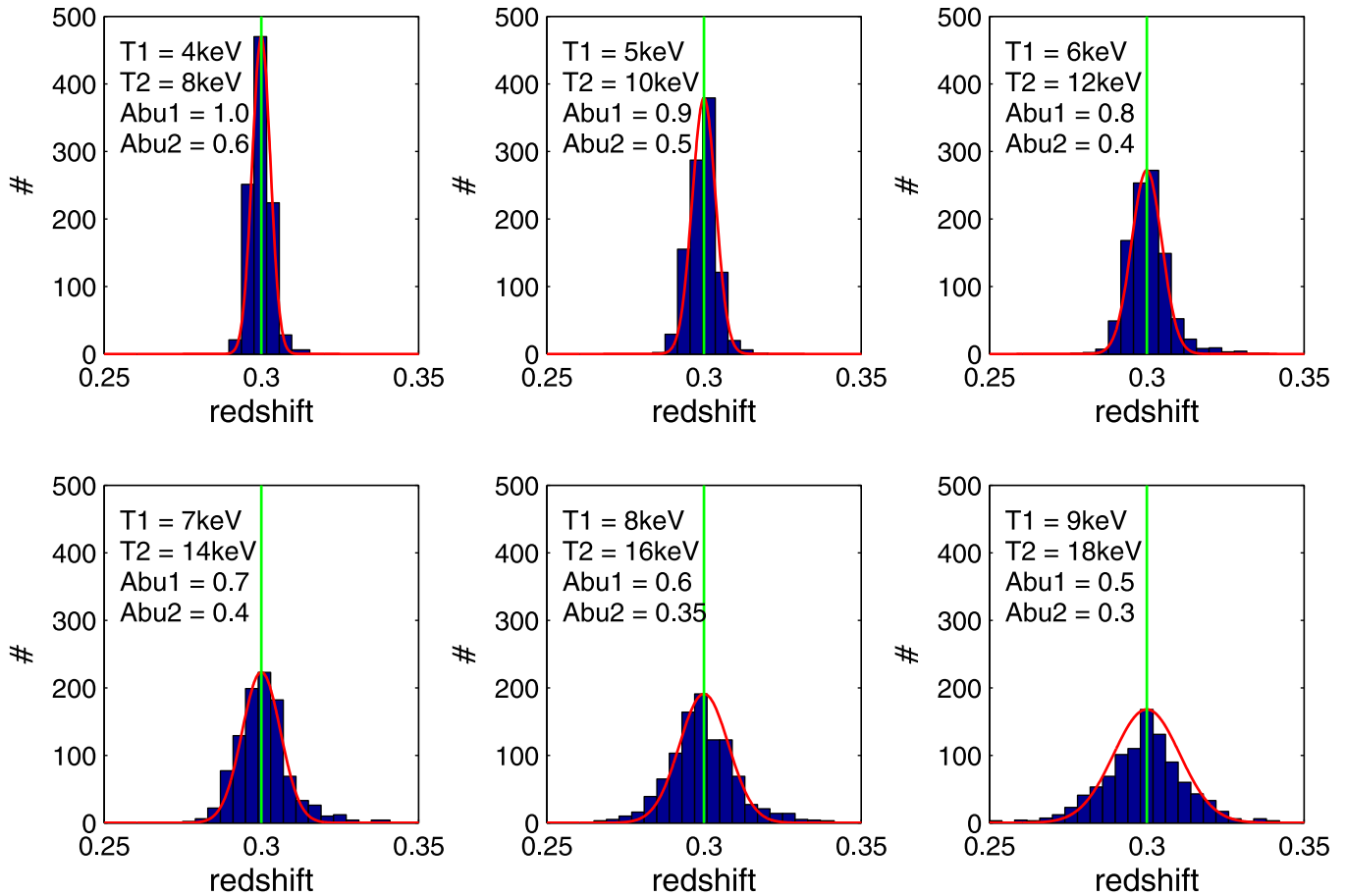
Figure 2. Histogram distribution of the best-fit redshift z_X for 10^3 simulated spectra with input temperature and abundances listed in Table 2 and z_{\text{input}} = 0.3 (shown with a green vertical line). In red, we show the Gaussian with amplitude \sigma_{\text{rms}} centered on \langle z_X \rangle .
