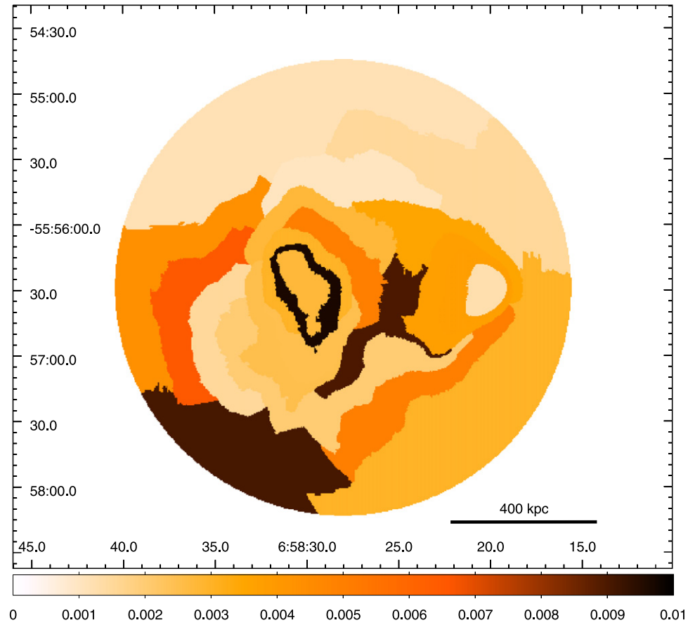
Figure 8. Map of the systematic 1\sigma error on the X-ray redshift z_X .
