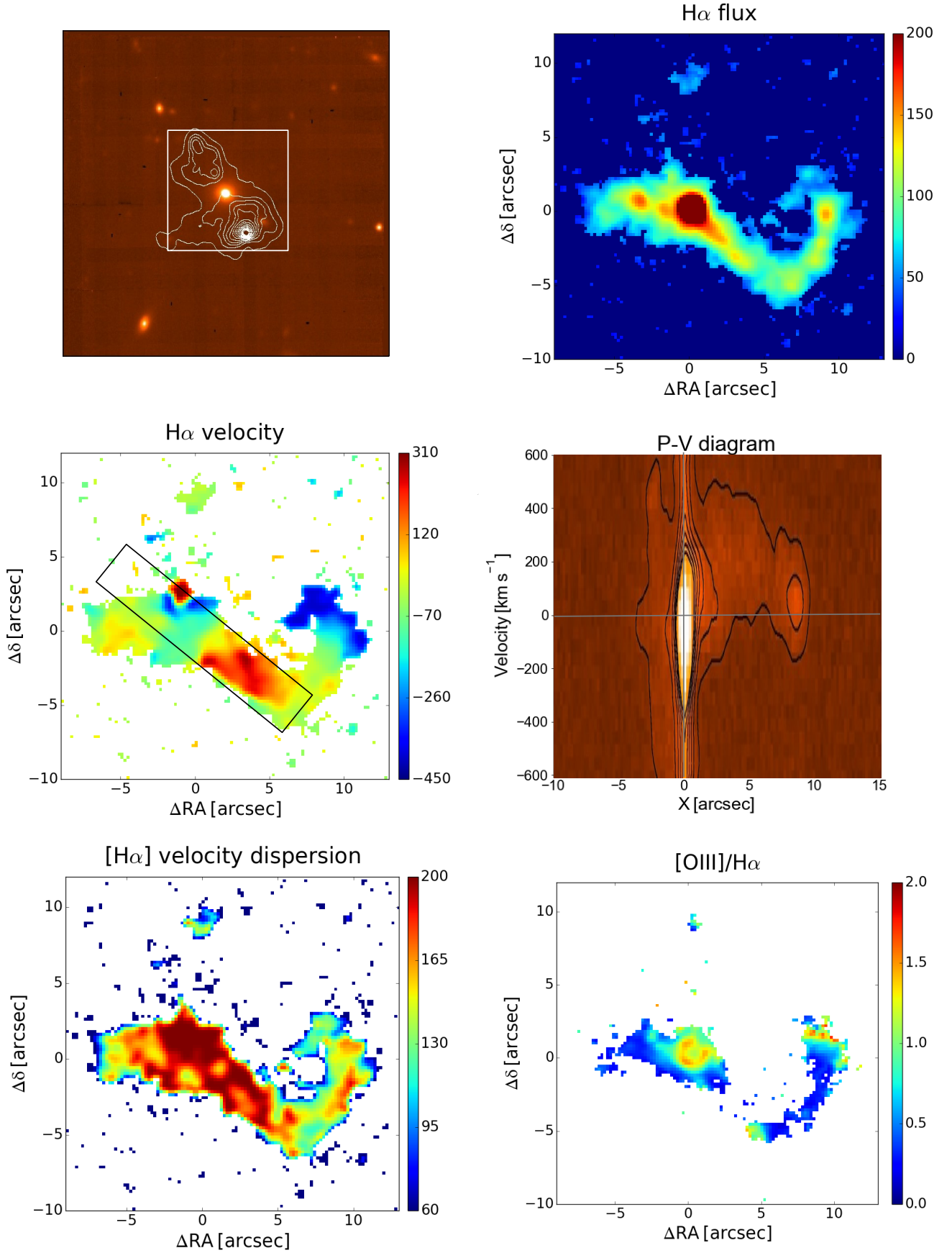
Fig. 7. 3C 063, FR II/HEG, 1'' = 2.99 kpc. Top left: radio contours overlaid onto the Muse optical continuum image. Top right: H \alpha emission line image extracted from the white square in the top left panel. Middle: velocity field from the H \alpha line and PV diagram (the synthetic slit is centered on the nucleus, has a width of 5 pixels and it is oriented at an angle of -60^\circ from the X axis). Bottom: H \alpha velocity dispersion and [O III]/H \alpha ratio.
