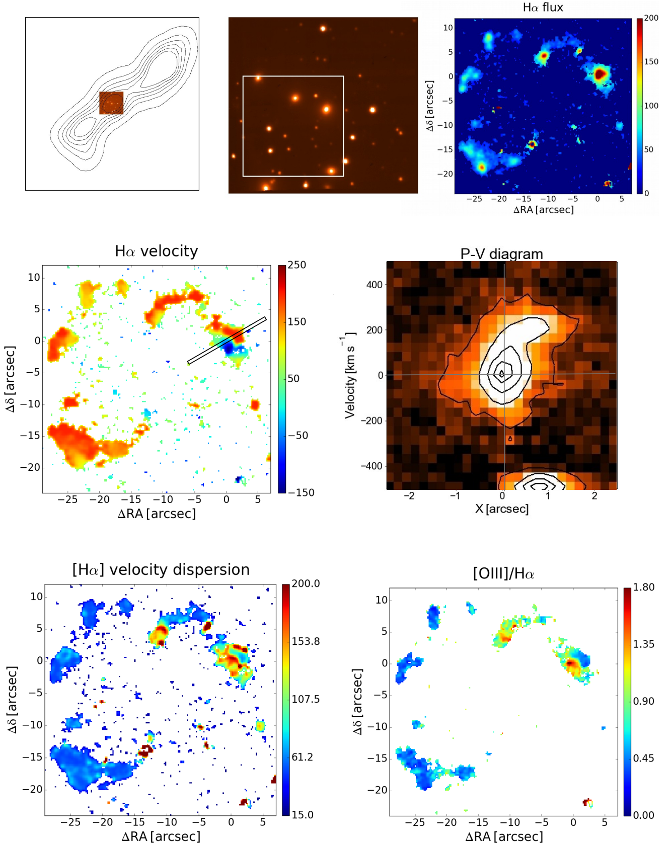
Fig. B.5. 3C 403.1, FR II/LEG, 1'' = 1.07 kpc. Top left: radio contours overlaid onto the Muse optical continuum image. Top center: Muse optical continuum image. Top right: H \alpha emission line image extracted from the white square in the top center panel. Middle: velocity field from the H \alpha line and PV diagram (the synthetic slit is centered on the nucleus, has a width of 5 pixels and it is oriented at an angle of 60^\circ from the X axis). Bottom: H \alpha velocity dispersion and [O III]/H \alpha ratio.
