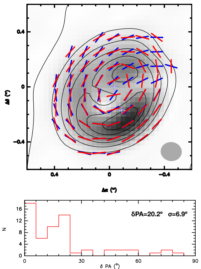
Fig. 7. Best fit for the polarization produced by radiation fields from the VLA 5a source (red vectors) and the Band 7 data (blue vectors). The grey scale indicates polarized intensity with same levels of Fig. 1. Vectors are shown for every 3 pixels. The position angle difference between the our data and the radiation alignment position angles are shown as a histogram in the bottom panel. The histogram bin is 6^\circ to be consistent with the largest observational uncertainty in position angle.
