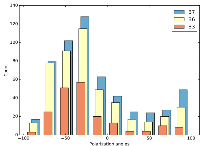
Fig. 3. Distribution of polarization angles for each band using a bin of 10^\circ .
