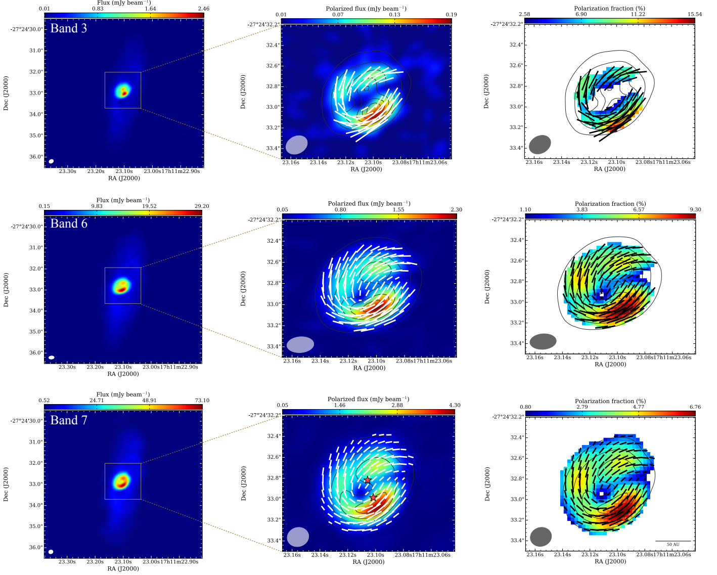
Fig. 1. Stokes I (left panel), polarized intensity (middle panel) and polarization fraction (right panel) of our Band 3 (upper panels), Band 6 (middle panels) and Band 7 (lower panels) ALMA data. The contours indicate the intensity levels of the Stokes I emission in each band, being 30, 60, 90, 120, 150, 180 times the rms for bands of 3 and 6 ( rms_{\text{Band 3}} \sim 0.012 mJy beam ^{-1} and rms_{\text{Band 6}} \sim 0.15 mJy beam ^{-1} ), and 30, 60, 90, 120 times 0.52 mJy beam ^{-1} , the rms for Band 7. The synthesized beams are 0.22'' \times 0.17'' (position angle = -61.46^\circ ) for Band 3, 0.26'' \times 0.15'' (position angle = -85.65^\circ ) for Band 6 and 0.21'' \times 0.18'' (position angle = -72.79^\circ ) for Band 7. The vector map indicates the orientation of the polarization whose length is proportional to the polarization fraction. The vectors are sampled as one vector every two pixels. The two star-symbols at the middle-lower panel indicate the position of the two continuum peaks detected in the 34 GHz VLA data, being VLA 5a the northern peak and VLA 5b the southern one (see also Fig. 2).
