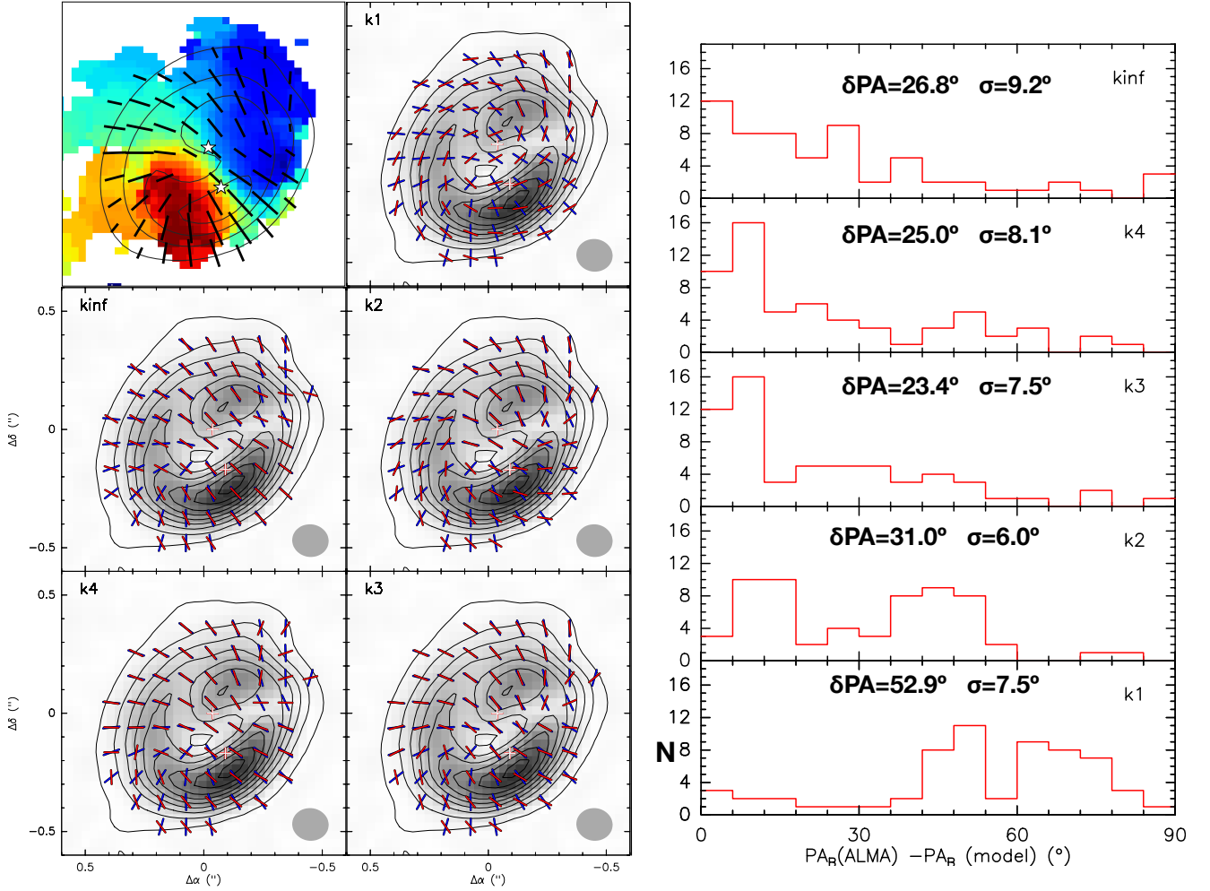
Fig. 8. Left panels show synthetic magnetic field lines (red vectors) plotted on top of observed Band 7 Stokes I contours (5 to 45 mJy beam -1 in steps of 5 mJy beam -1 ), polarized intensity (grey scale with same intensity levels of Fig. 1) and magnetic fields (blue vectors, which are 90°-rotated with respect to Fig. 1). The red vectors result from our rotating disk modeling assuming different k = B_p/B_\phi values. Fig. 6 is shown in the upper left panel for reference. The right panels show the residuals from each case, with mean \delta\text{PA} = \text{PA}_{\text{data}} - \text{PA}_{\text{model}} values and standard deviation \sigma indicated on each histogram panel.
