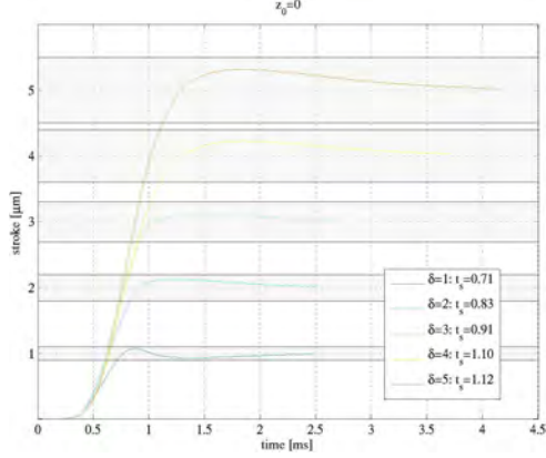
Figure 9: Step response when z_0 = 0 . The shaded strips indicate the areas where |(z - \delta)/\delta| \leq 10\% .
