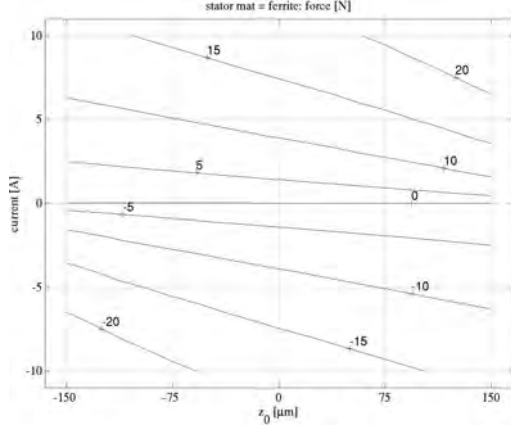
Figure 5: Force vs current and position (see text for a discussion).
