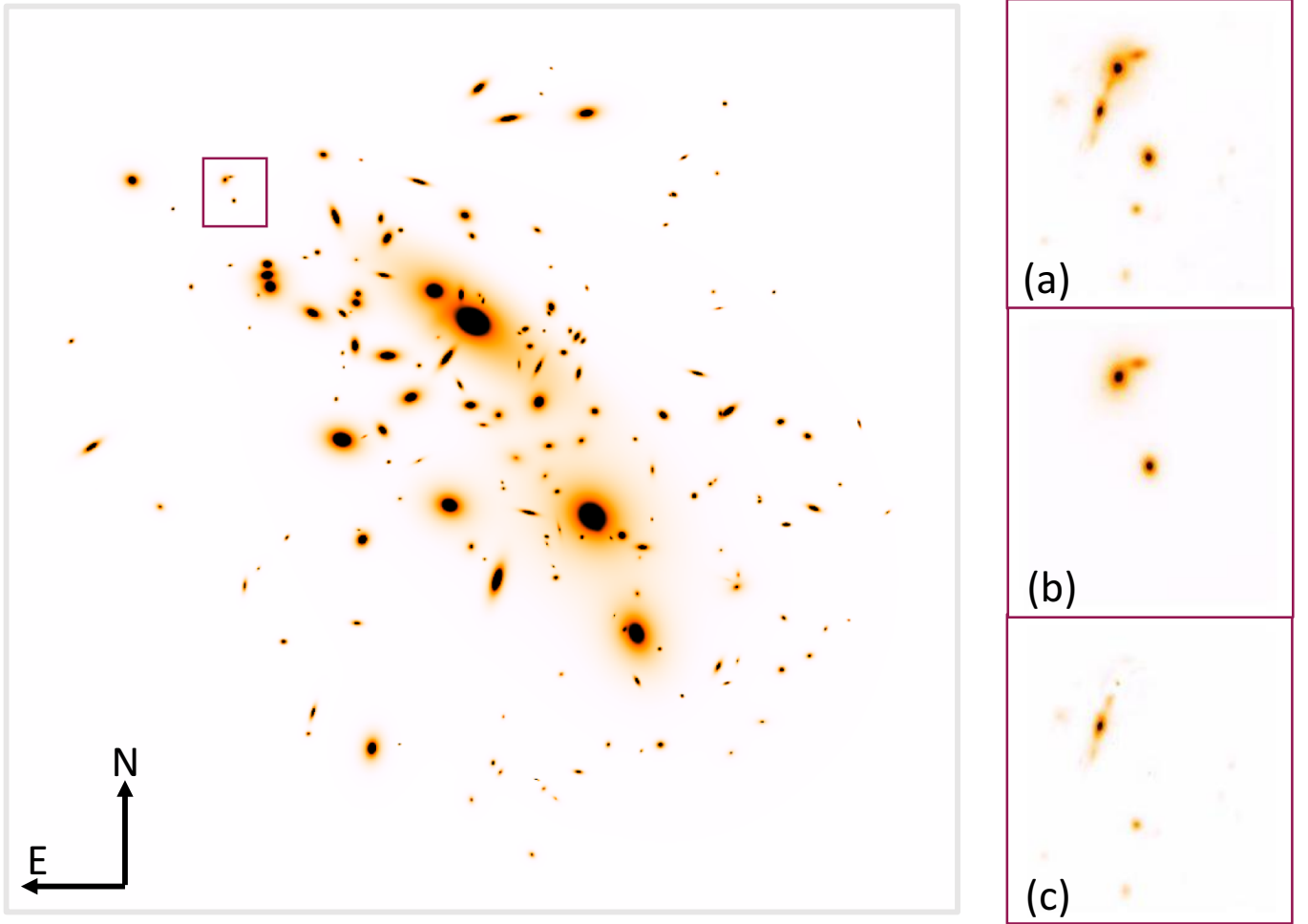
Figure 1. Left: Model image of all cluster members before the convolution with the PSF. The image is 2 \times 2 arcmin and covers the entire HST field of view. Right: Original, model and residual images of some interacting sources (top, middle and bottom panel respectively) corresponding to the selection box in the main image ( \sim 9 \times 9 arcsec). The seven sources in the original and residual images are foreground/background galaxies which have not been modeled.
