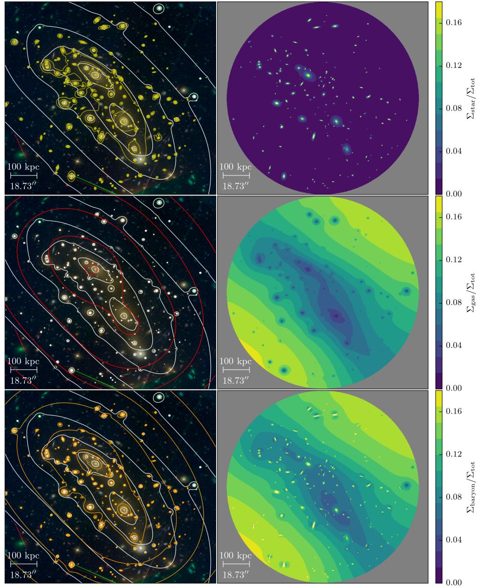
Figure 2. Left panels: total, stellar, hot gas and baryonic surface mass density isocontours overlaid on a color-composite image of the cluster in 7 optical filters. White lines are the total mass isodensity levels which have a logarithmic step between 0.00035 and 0.003 \text{ M}_\odot/\text{kpc}^2 . Yellow lines refer to the stellar mass isodensities and are spaced between 3.5 \times 10^{-6} to 3 \times 10^{-4} \text{ M}_\odot/\text{kpc}^2 . Red lines are the hot gas isodensity contours spaced between 4.5 \times 10^{-5} and 1.8 \times 10^{-4} \text{ M}_\odot/\text{kpc}^2 . Orange lines refer to the baryonic component (stars + hot gas) and have the same range as the hot gas component. Right panels show the two-dimensional surface density profile ratios of stellar (upper panel), hot gas (middle panel) and baryon (bottom panel) over total mass.
