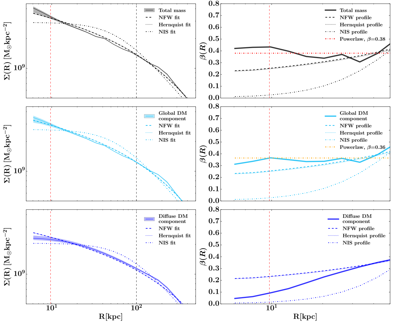
Figure 4. Left Panels: Surface mass density profiles of total (top row) and dark-matter (middle and bottom rows) components fitted with a NFW (Navarro et al. 1996), Hernquist (Hernquist 1990) and a softened isothermal sphere (NIS; Grogin & Narayan 1996) profile. Right panels: \beta(R) as defined as in Eq. 1 calculated for the total (top row) and dark matter (middle and bottom rows) surface mass densities and compared with the values of NFW (dashed), Hernquist (dotted), softened isothermal sphere (dot-dashed), fits. The red dashed lines show the effective radius of the BCG. The black dashed lines represent the radius where we see a change in the slope of the total surface mass density profile and represents also the range in which we have performed a fit with a power-law profile. To better show the differences, in the right panels we focus on the inner 50 kpc.
