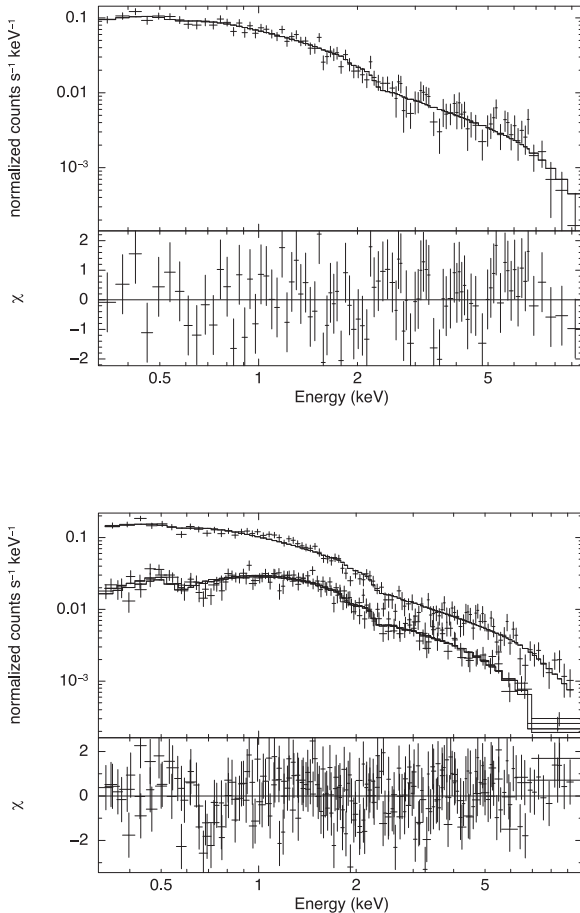
Figure 6. EPIC spectra and residuals of PKS 2004–447 fitted with a power law. For the first observation (upper panel) only EPIC-pn data were considered, while for the second (bottom panel) EPIC-pn, MOS1, and MOS2 were considered in the fit.
