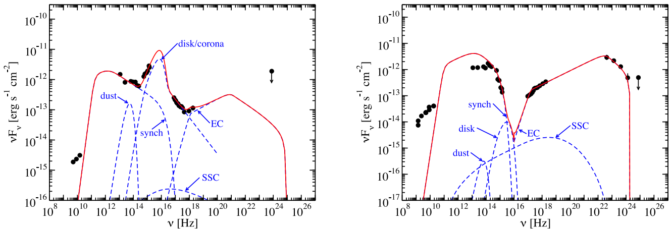
Figure 8. SED data (circles) and model fit (solid curve) of J1548+3511 (left) and PKS 2004–447 (right). The model components are shown as dashed curves. Multiwavelength data are not simultaneous.
