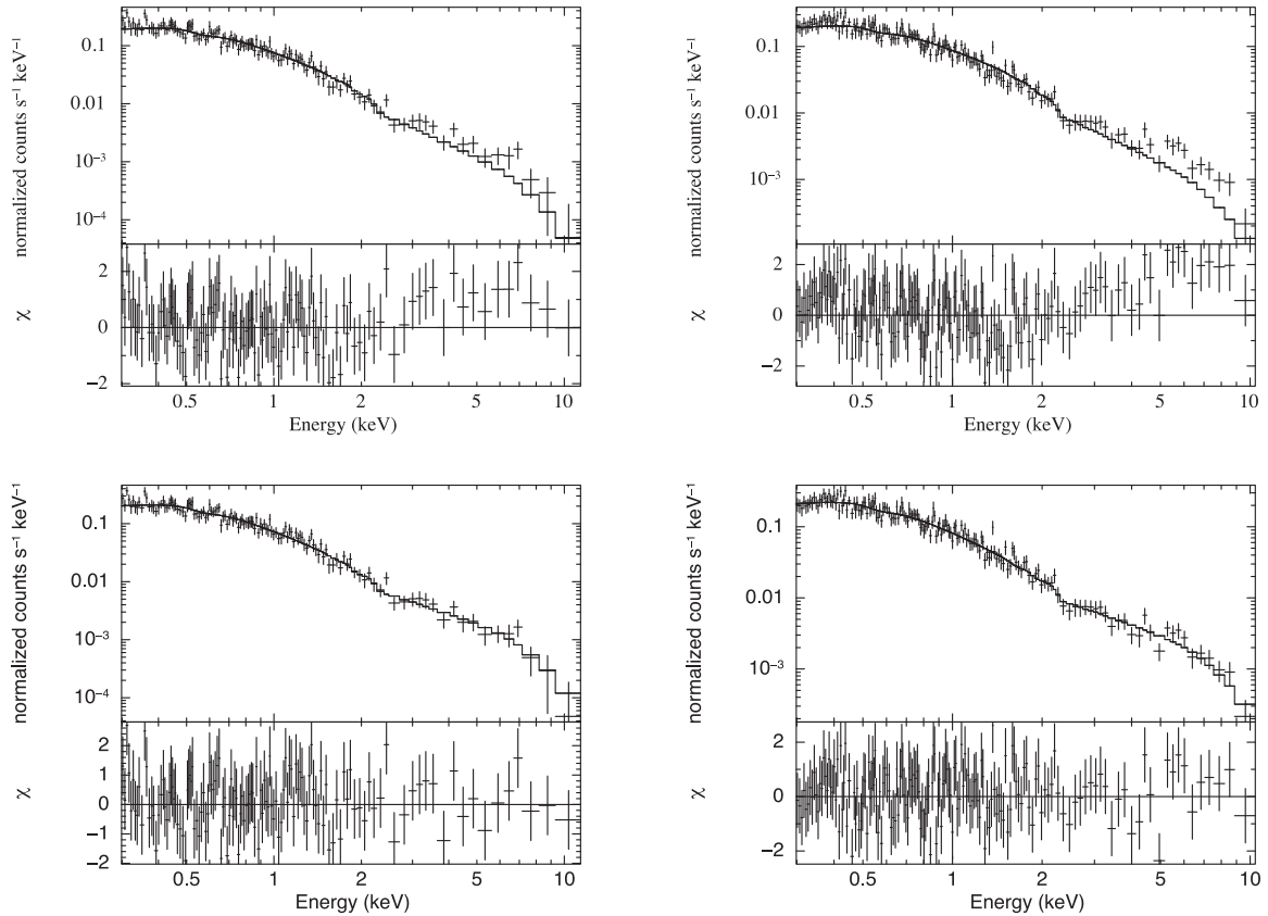
Figure 5. EPIC-pn spectra and residuals of J1548+3511 fitted with a power law (upper panel) and a broken power law (lower panel). The first observation is shown to the left and the second one to the right.
