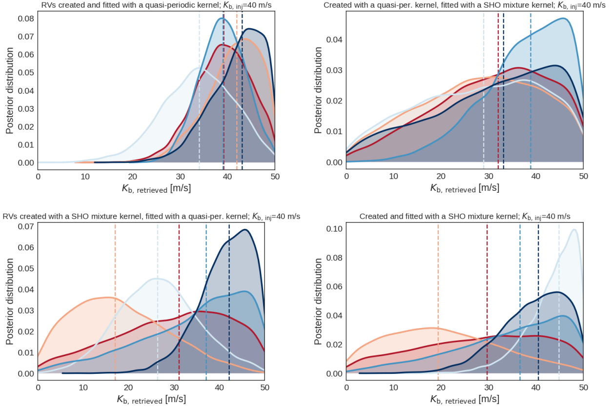
Fig. 8. Posteriors of the K_b parameter retrieved from the simulations involving mock RV datasets build on the best-fit stellar activity signals based on a quasi-periodic and SHO mixture models (see the text for details). The simulated RV time series include an injected planetary signal of semi-amplitude K_{b,\text{inj}} = 40 \text{ m s}^{-1} . Only five out of a total of ten posteriors are shown for the sake of a better readability. First row: results from the fit of data generated using a quasi-periodic kernel. Second row: results from the fit of data generated using a SHO mixture kernel. In both rows, each colour identifies one mock dataset, therefore, the posterior distributions with the same colour can be compared. The vertical lines indicate the median of the posteriors.
