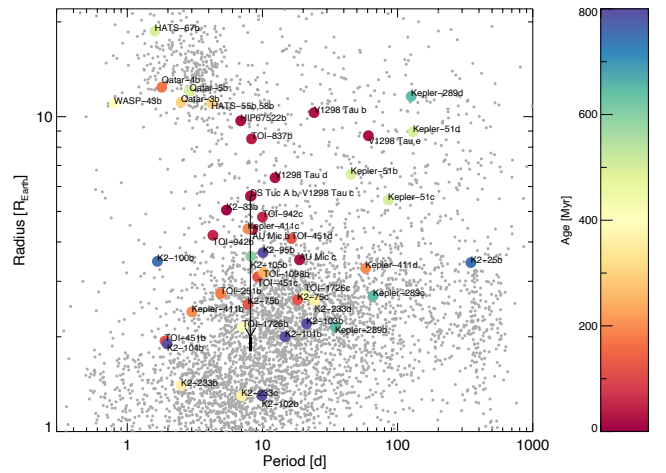
Fig. 19. Planetary period-radius diagram for the sample of characterised young transiting planets as a function of the stellar age. Grey dots represent all the known planets with measured period and radius. Black bar line indicates the locus of the final radius of DS Tuc A b according to our planetary evolution models.
