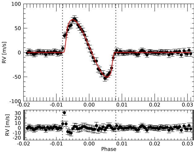
Fig. 10. RM effect for DS Tuc A b from ESPRESSO data modelled by our fit (red line) with the corresponding residuals. Vertical dotted lines indicate the transit ingress and egress.
