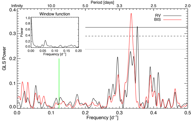
Fig. 3. GLS of the HARPS RV (black line) and BIS (red line) time series of DS Tuc A. The green vertical line indicates the location of the planet orbital period, while the window function of the observations is reported in the inset plot. Dotted, dashed, and solid black horizontal lines indicate the FAP thresholds at 1, 0.1, and 0.01%, respectively, for the RV periodogram.
