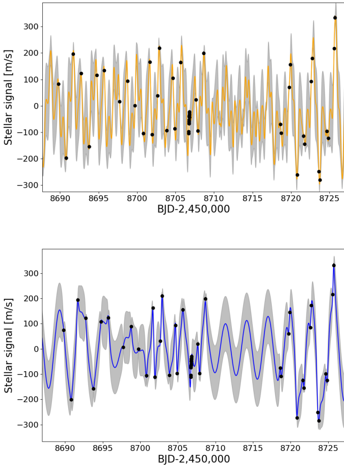
Fig. 6. Summary of the GP best-fit model as obtained from the joint analysis of the HARPS+ESPRESSO RVs. Here, we show a portion of the HARPS time series, after removing the best-fit signal induced by planet b. The shaded area in gray represents the \pm 1\sigma confidence interval. Upper panel: best-fit model for the GP quasi-periodic kernel (orange line). Lower panel: same as above, but for the GP rotation kernel (blue line).
