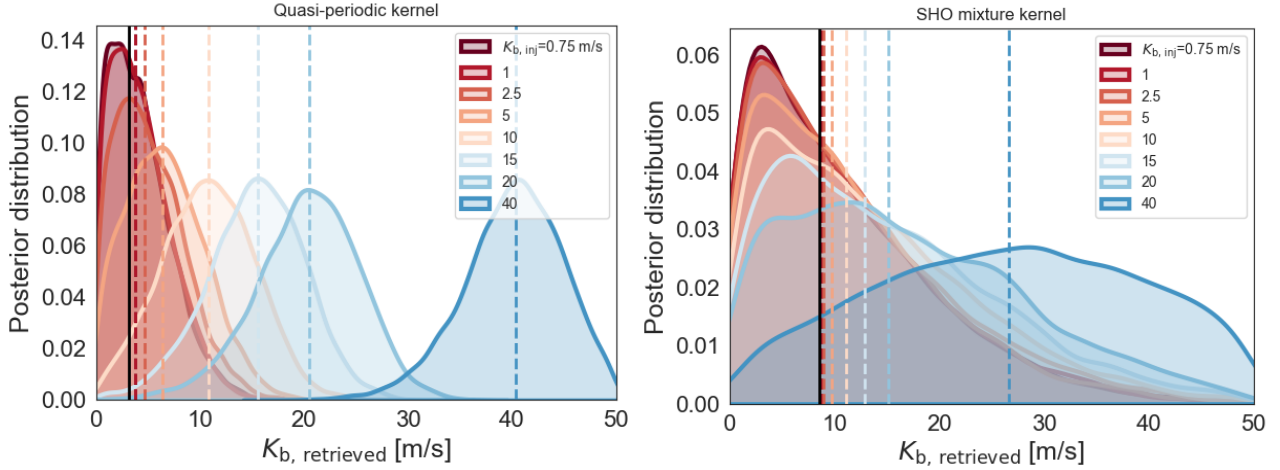
Fig. 7. Posteriors of the K_b parameter retrieved from the simulations involving the original RV datasets, with the injected K_{b, \text{inj}} values indicated in the legend. The vertical dashed lines represent the median of the posteriors of the corresponding colour. The vertical black lines indicates the median of the posteriors for the real data ( 3.2 and 8.6 \text{ m s}^{-1} ), as a reference.
