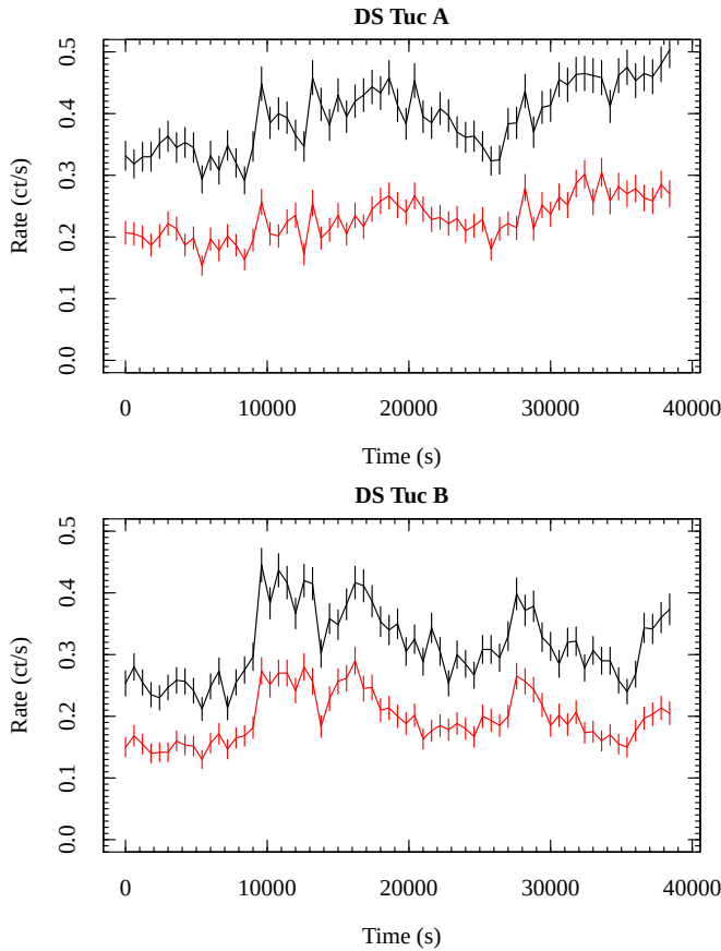
Fig. 15. Mos1 light curves for both components of DS Tuc. Black line is the light curve from the semi-circular region of radius 30'' , red line is the light curve from the circular region of radius 10'' . Error bars on rates are at 68% confidence level. Upper panel: DS Tuc A. Lower panel: DS Tuc B.
