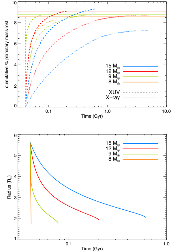
Fig. 17. Summary of our simulations on the atmospheric evolution of DS Tuc A b. Upper panel: cumulative percentage of the planetary mass loss evolution considering the X+EUUV irradiation (dashed) or X-ray irradiation alone (dotted). We used the results obtained with the evolution by Penz et al. (2008) . Horizontal solid lines represent the limits of the atmospheric mass concerning four representative cases with different starting masses, colour-coded as in the legend. Lower panel: radius evolution corresponding to the representative cases according to our models from the present age of the system to the end of the photo-evaporation phase.
