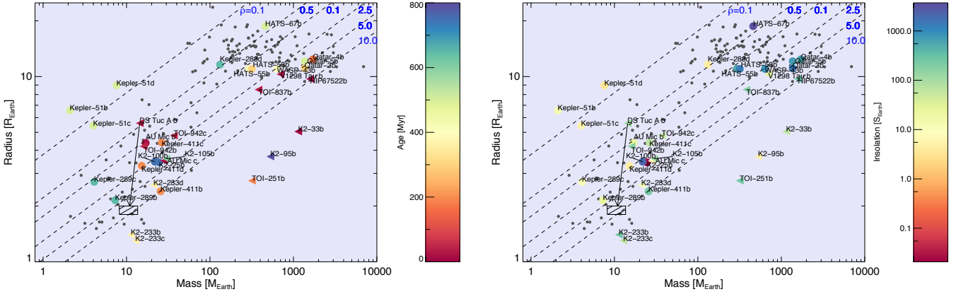
Fig. 18. Planetary mass-radius diagram for a sample of characterised young transiting planets as a function of the stellar age ( left ) and planet insolation ( right ). Coloured circles indicate planet with measured mass, while triangles indicate planets with mass upper limit only. Grey dots represent a sample of well-characterised mature exoplanets for comparison. Dashed lines represent loci of equal density, as indicated at the top of the figure. Hatched rectangle indicates the locus of the final mass and radius of DS Tuc A b, according to our planetary evolution models.
