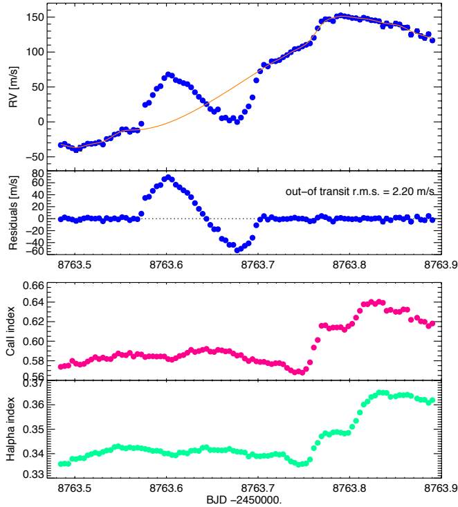
Fig. 9. Radial velocities and activity indices variation during the transit of Oct. 6 of DS Tuc A b observed with ESPRESSO. Upper panel: RV (blue dots) with the GP model of the stellar activity (orange line) and the corresponding residuals. Lower panel: Call H&K and H\alpha time series extracted from the same spectra.
