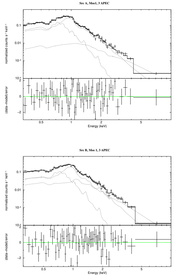
Fig. 16. X-ray spectra of DS Tuc A ( upper panel ) and DS Tuc B ( lower panel ). Each panel is subdivided in two plots: spectrum with the best fit model (a sum of 3 APEC components, each one indicated by the dotted lines) and the terms of \chi^2 for each bin in units of \chi^2 standard deviation.
